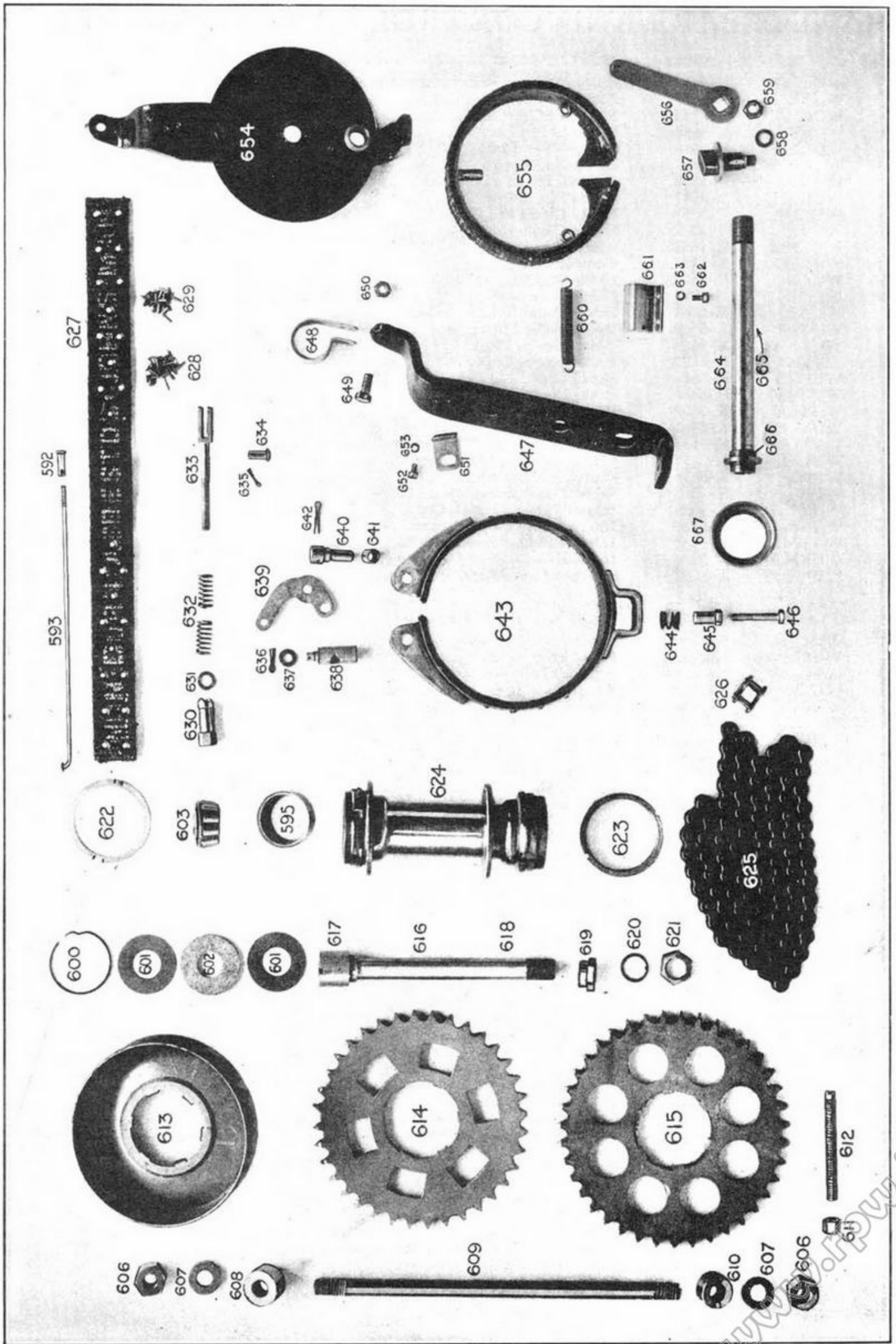
X—BRAKE AND REAR WHEEL PARTS
