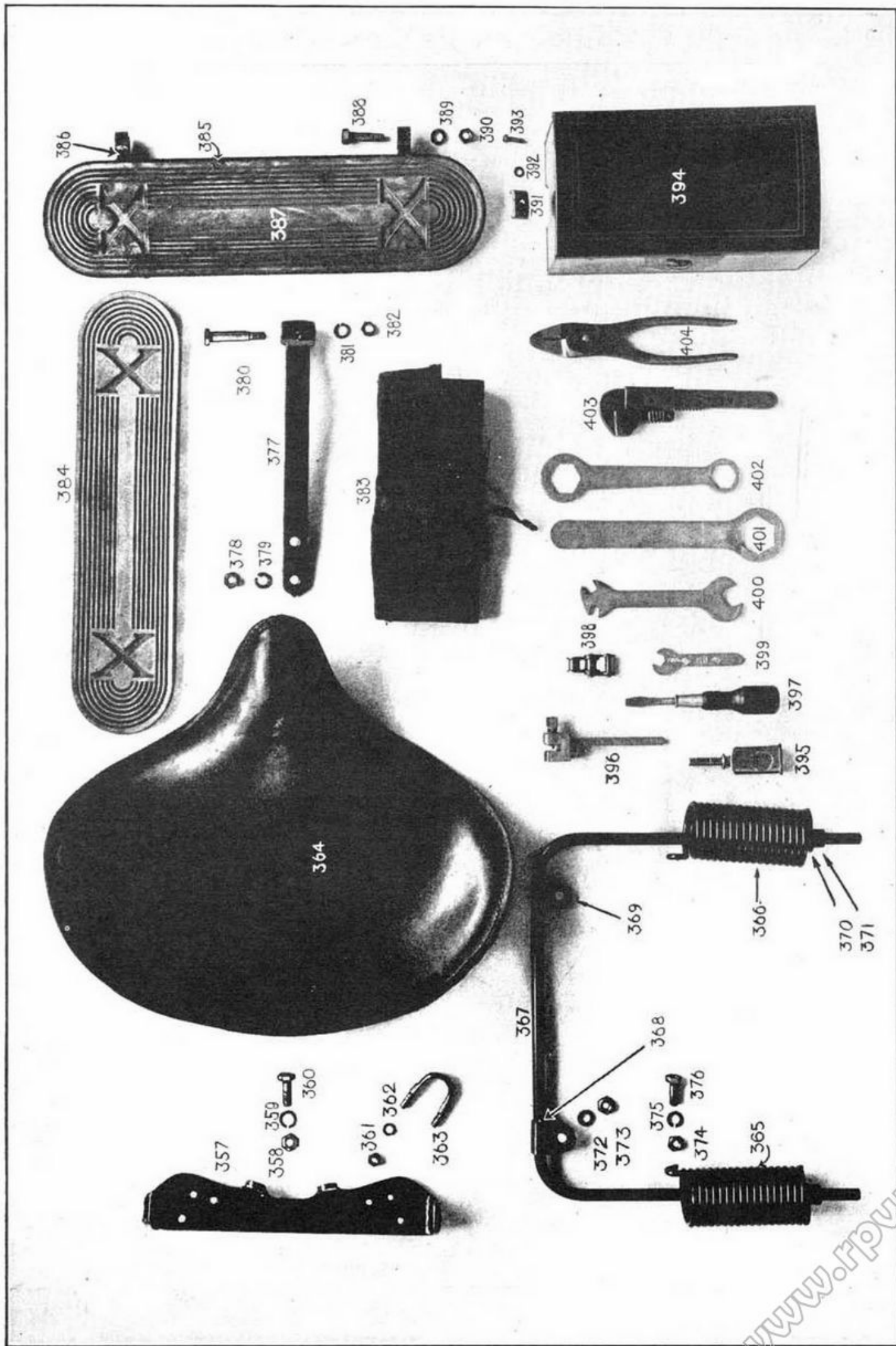
VI—SADDLE, TOOL KIT AND FOOT BOARDS
