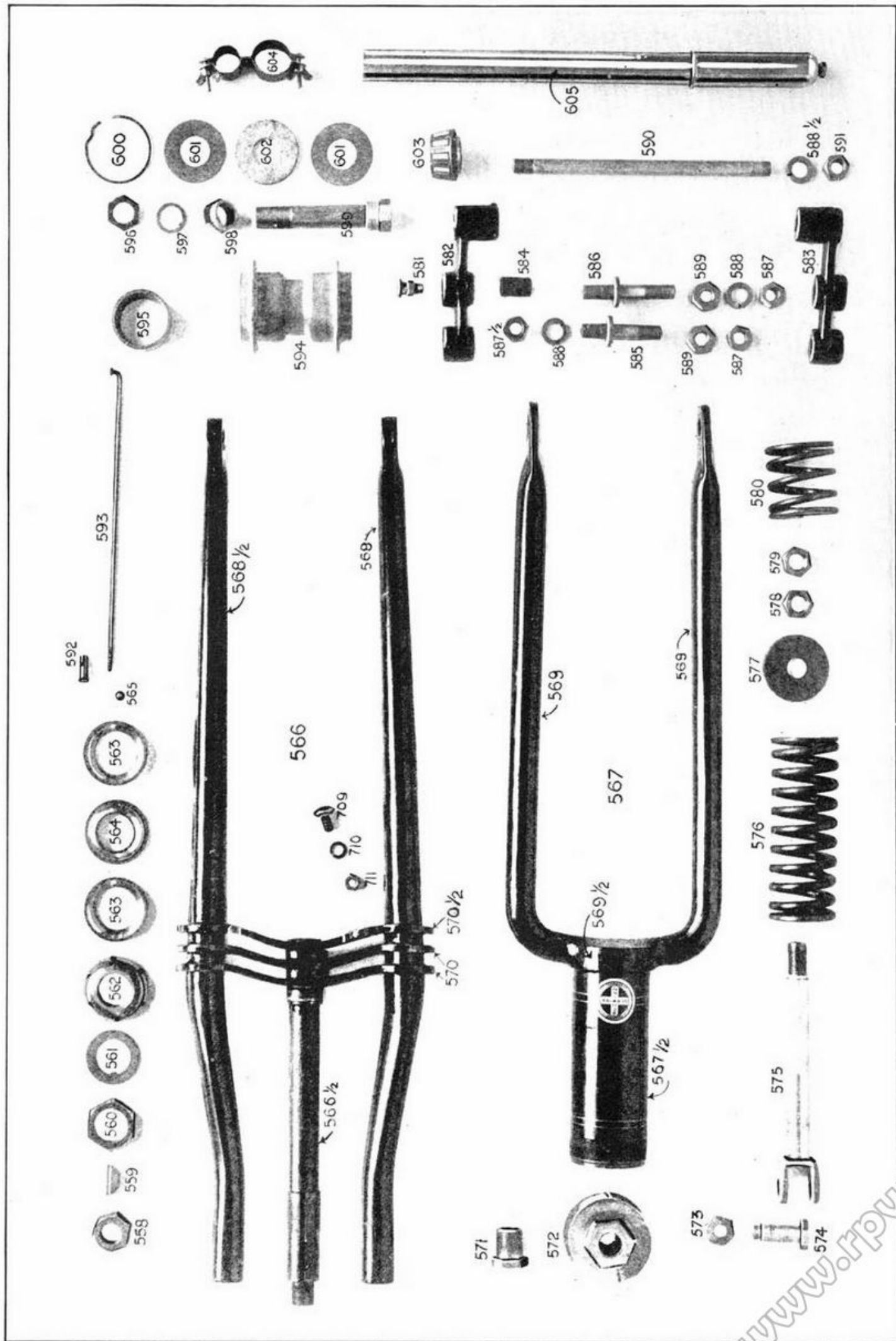
IX—FORK AND FRONT WHEEL PARTS
