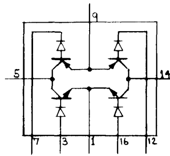
TM EGC-101 EQUIVALENT CIRCUIT U.S. PATENT #3,714,462 OTHER PATENTS PENDING
