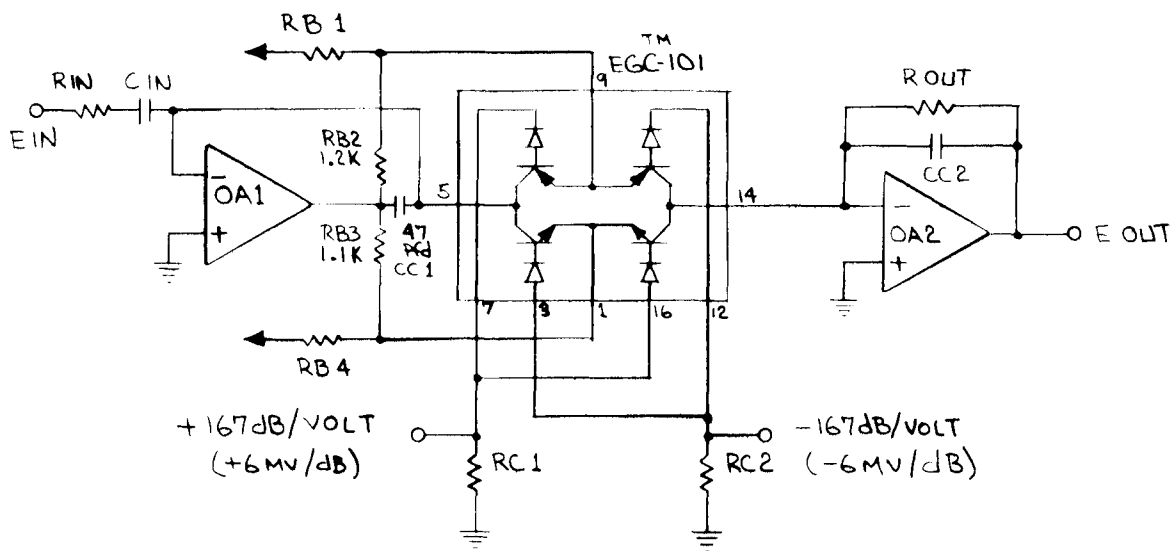
TM BASIC VCA UTILIZING EGC-101 U.S. PATENT #3,714,462 OTHER PATENTS PENDING FIGURE 3
