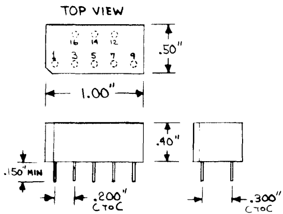
.025" DIA LEADS 8 PLACES TIN ON COPPER ON STEEL FIGURE 1
