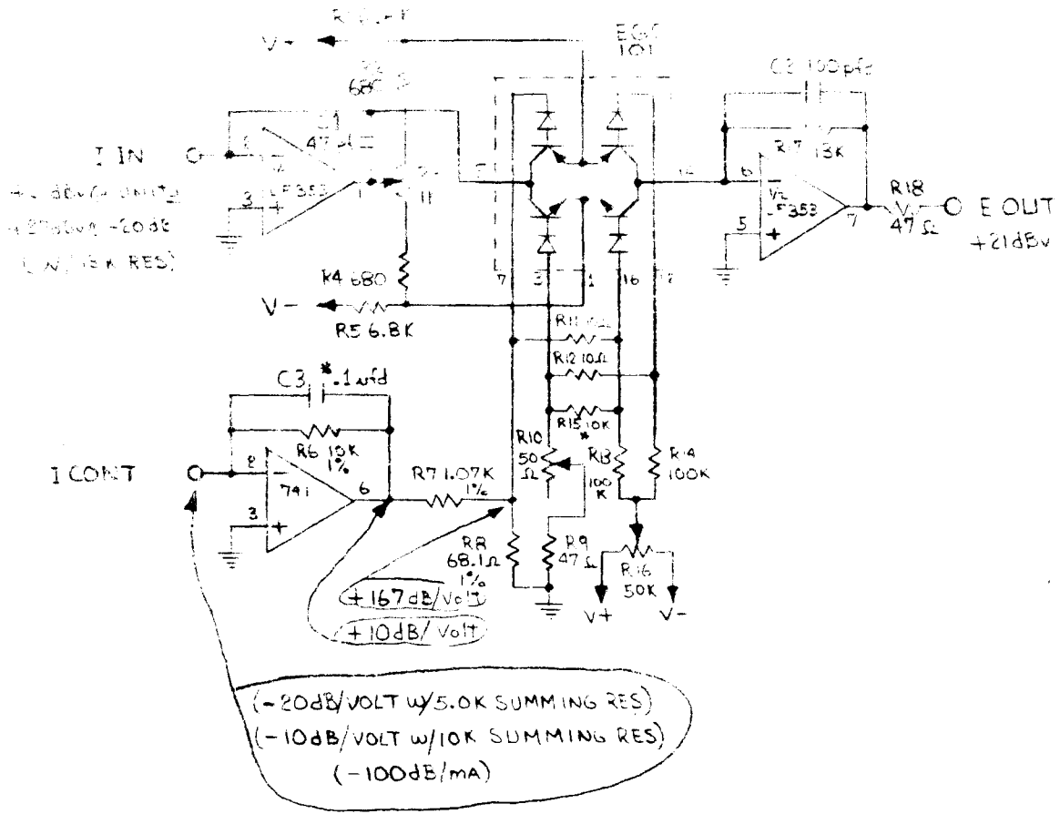
EGC-205M (FULLY TRIMMED VCA CKT WITH CURRENT INPUTS & VOLTAGE OUTPUT) US PATENT # 3,714,462 AND OTHER PATENTS PENDING FIGURE 4
