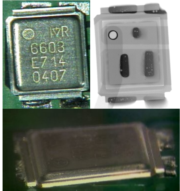
Figure 10 Twisted and tilted device
