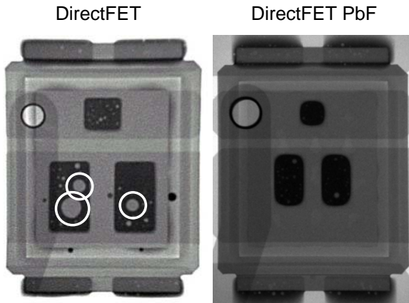
Figure 11 Examples of solder voids
