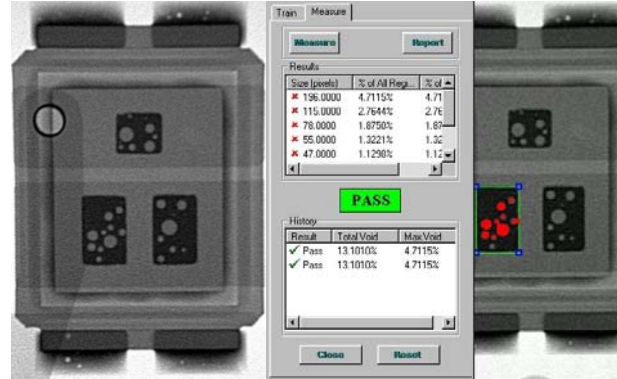
Figure 13 Voids on the left source contact
