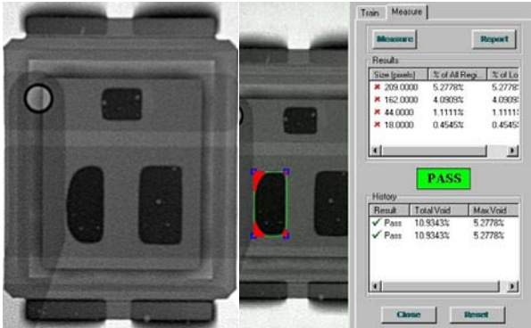
Figure 18 Poorly formed source joint – 11% missing
