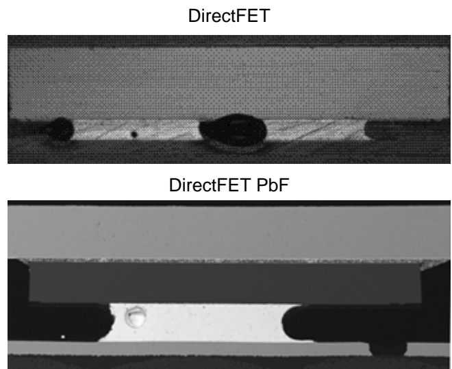
Figure 17 Cross-sectional views of solder joints
