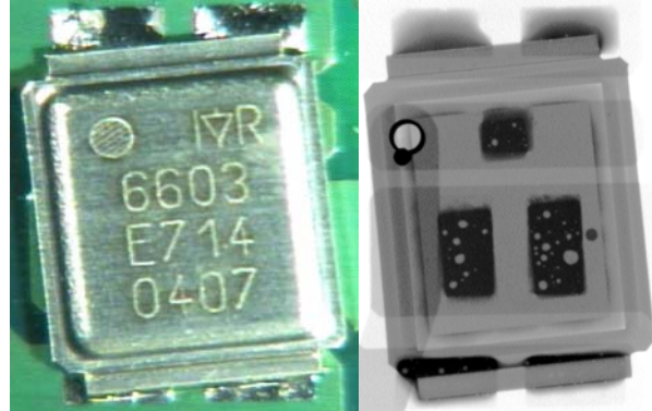
Figure 7 Twisted device
