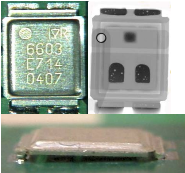
Figure 9 Tilted device
