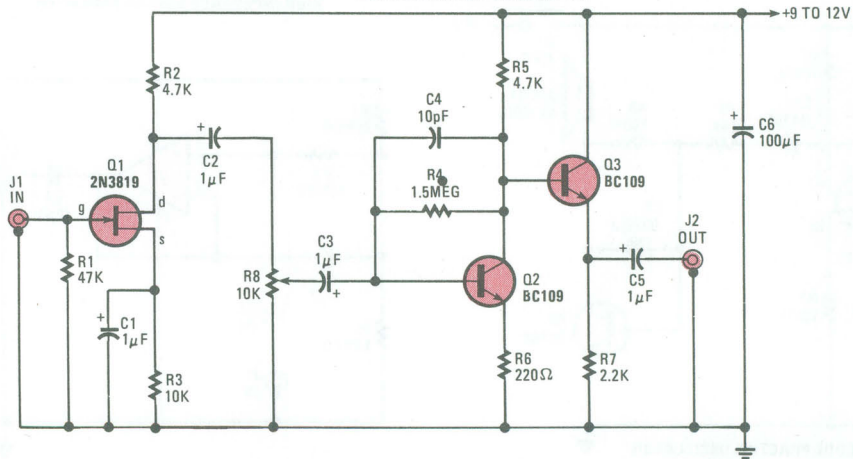
50K MICROPHONE PREAMPLIFIER
