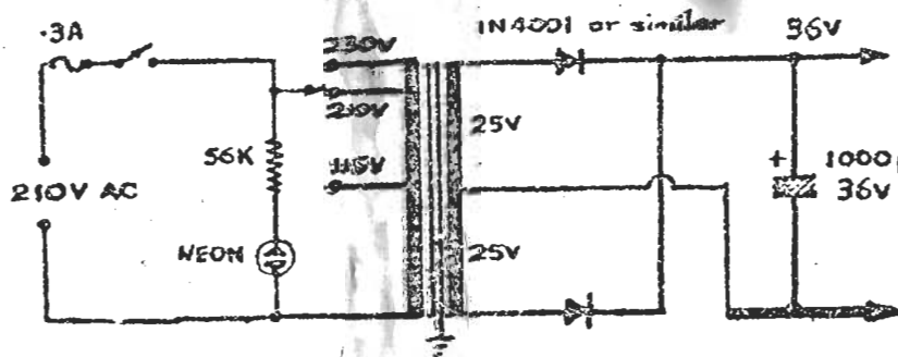
SUGGESTED POWER SUPPLY UNIT (NOT SUPPLIED IN SP175 KIT)
