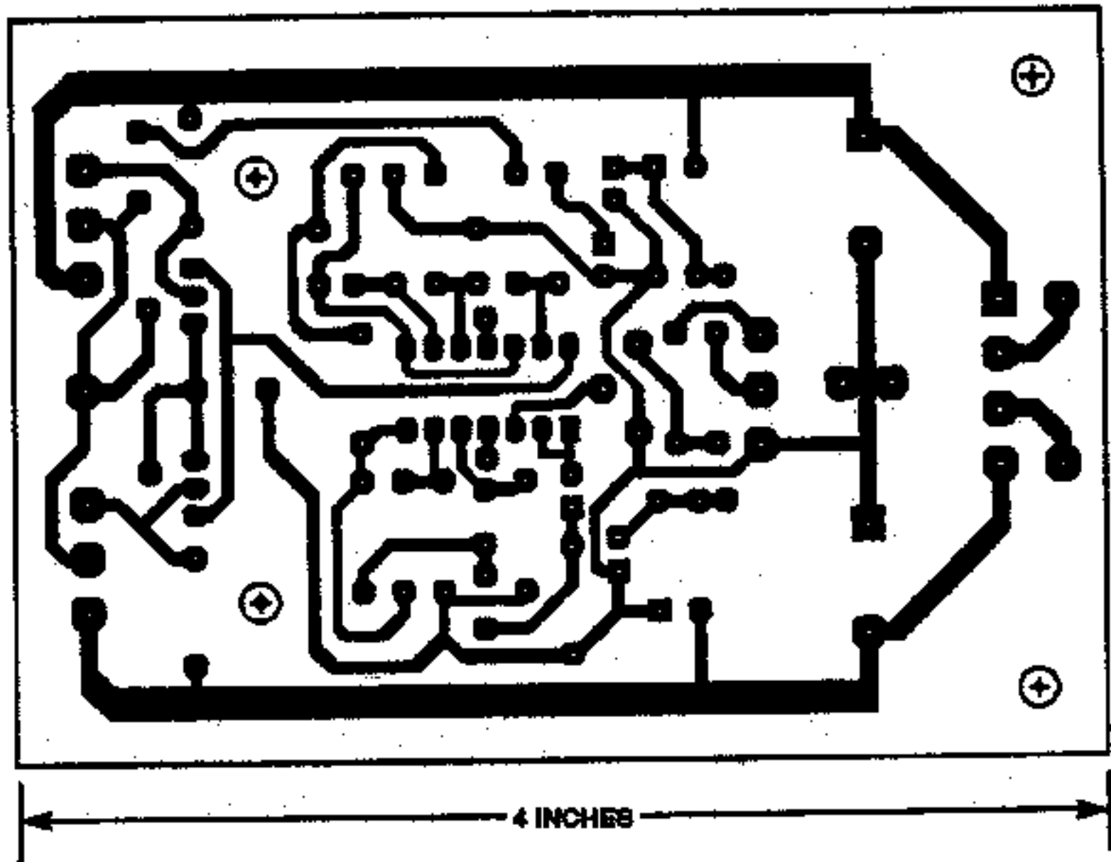
FOIL PATTERN for the amplifier/crossover board.
