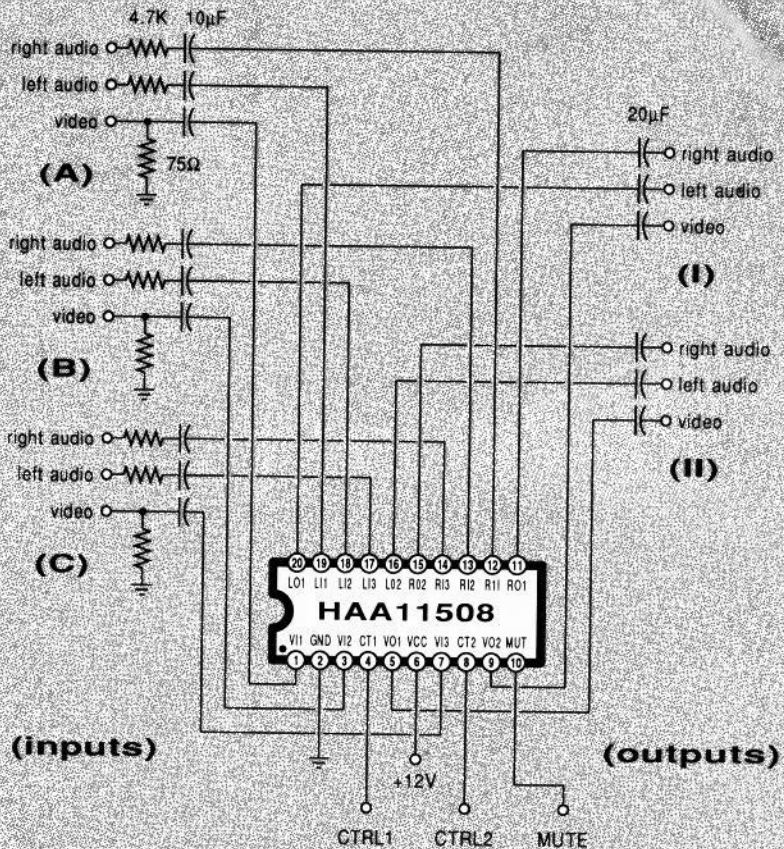
FIG. 1—THIS TRIPLE AUDIOVISUAL SWITCHER uses the Hitachi HAA11508 to simultaneously select video and two-channel stereo audio from any one of three sources and then route them to one of two selected outputs.
