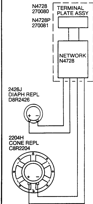
4728P WIRING SCHEMATIC, PASSIVE CROSSOVER
