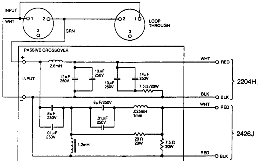
4728P WIRING SCHEMATIC, PASSIVE CROSSOVER
