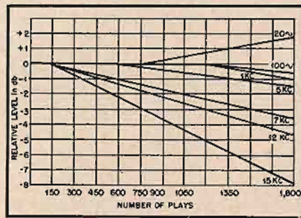
Fig. 4. Behavior of playback level of tape samples containing individual sine-wave components during 1800 replays.
