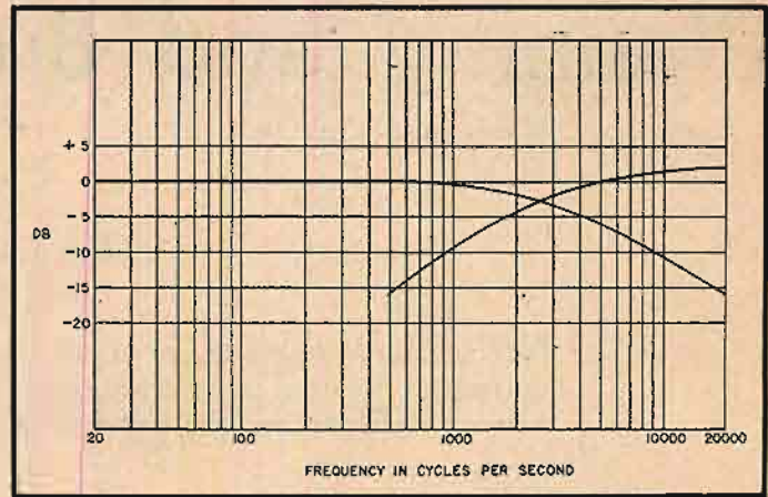
Fig. 6. The measured frequency characteristic of the crossover network.
