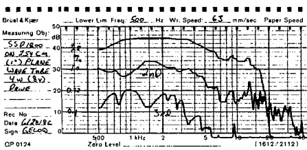
Harmonic Distortion with 4 w input
