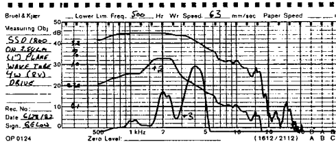
Intermodulation Distortion at 4 w Input
