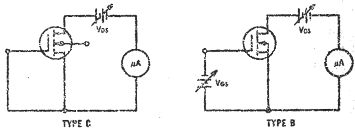
FIGURE 12b - V_{(BR)GSS} and V_{(BR)DSX} Test Circuit (Usually Used for MOSFETs Only).
