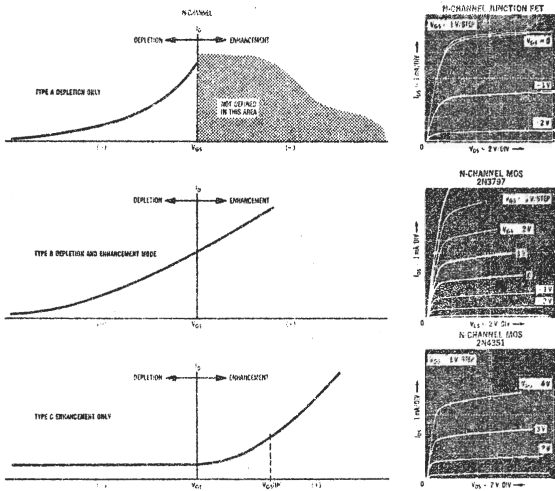
FIGURE 9 — Transfer Characteristics and Associated Scope Traces for Types A, B and C FETs
