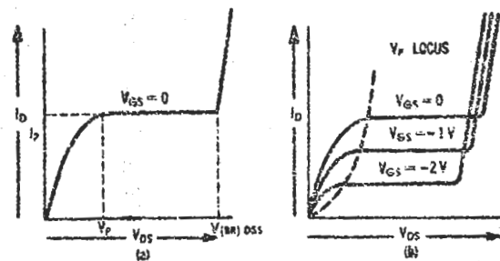
FIGURE 2 — Drain Current Characteristics
