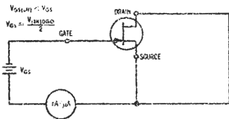
FIGURE 11 - Test Circuit for Leakage Current
