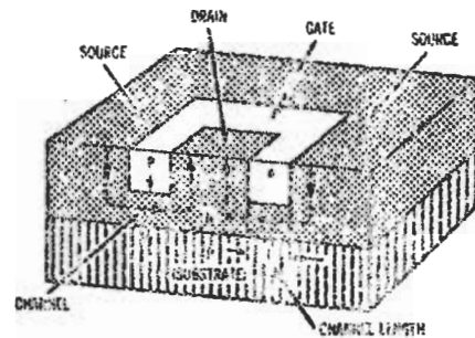
FIGURE 3 - Junction FET with Single-Ended Geometry
