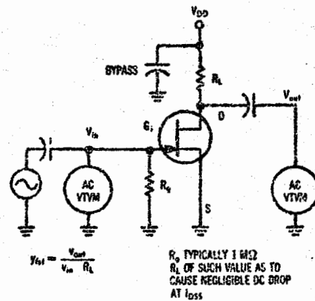
FIGURE 13 -- Typical y_{fs} Test Circuit
