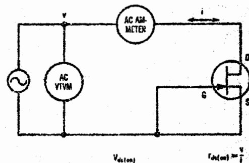
FIGURE 20 - Circuit for Measuring JFET Channel Resistance
