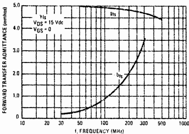
FIGURE 15 — Forward Transfer Admittance versus Frequency
