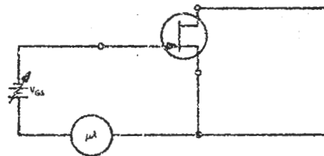
Figure 12a - V_{(BR)GSS} Test Circuit
