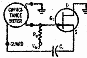
(a) V_{GS} = -V_{DS} R_g TYPICALLY 1 M \Omega C_c AC SOURCE TO GUARD SIGNAL.
