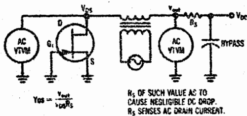
FIGURE 16 — y_{os} Measurement Circuit for Type A and B FETs
