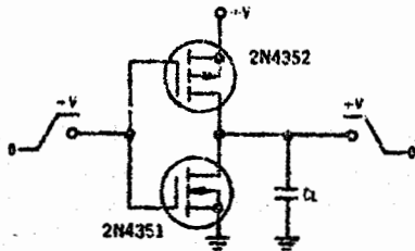
FIGURE 23 — Complementary Inverter Circuit
