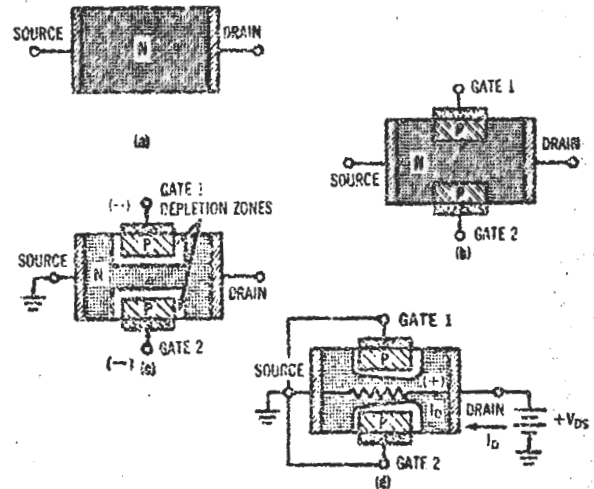
FIGURE 1 — Development of Junction Field-Effect Transistors
