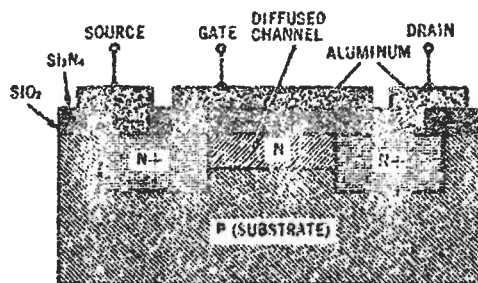
FIGURE 7 - Depletion Mode MOSFET Structure. This Type of Device may be Designed to Operate in Both the Enhancement and Depletion Modes
