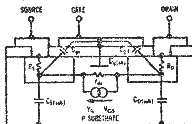
FIGURE 6 - Equivalent Circuit of Enhancement-Mode MOSFET
