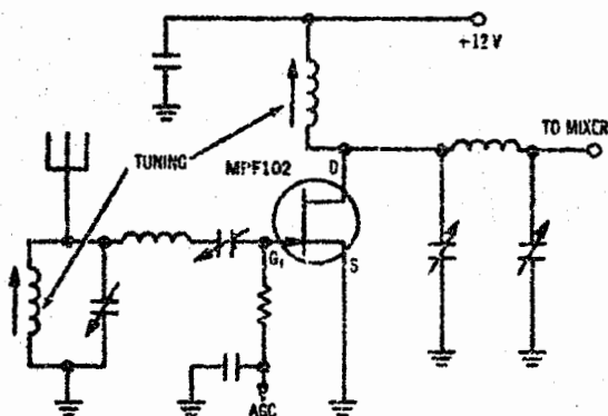
FIGURE 21 - RF Stage of Broadcast Auto Radio
