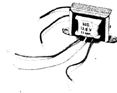
Fig. 1. Typical filament transformer has current and voltage ratings printed on side providing data needed to calculate wire size and turns ratio modifications for constructing a transformer with different voltage, impedance or power rating.
