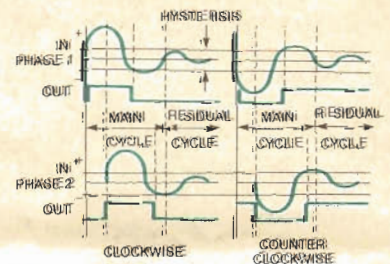
FIG. 12—COMPARATOR WAVEFORMS. The hysteresis trip points are set to less than the peak amplitude of the main cycle of the sinewave, but greater than the peak value of the residual cycle.
