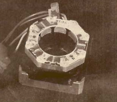
FIG. 2—THIS DISASSEMBLED 200 step/revolution stepper motor has 50 teeth in each row.
