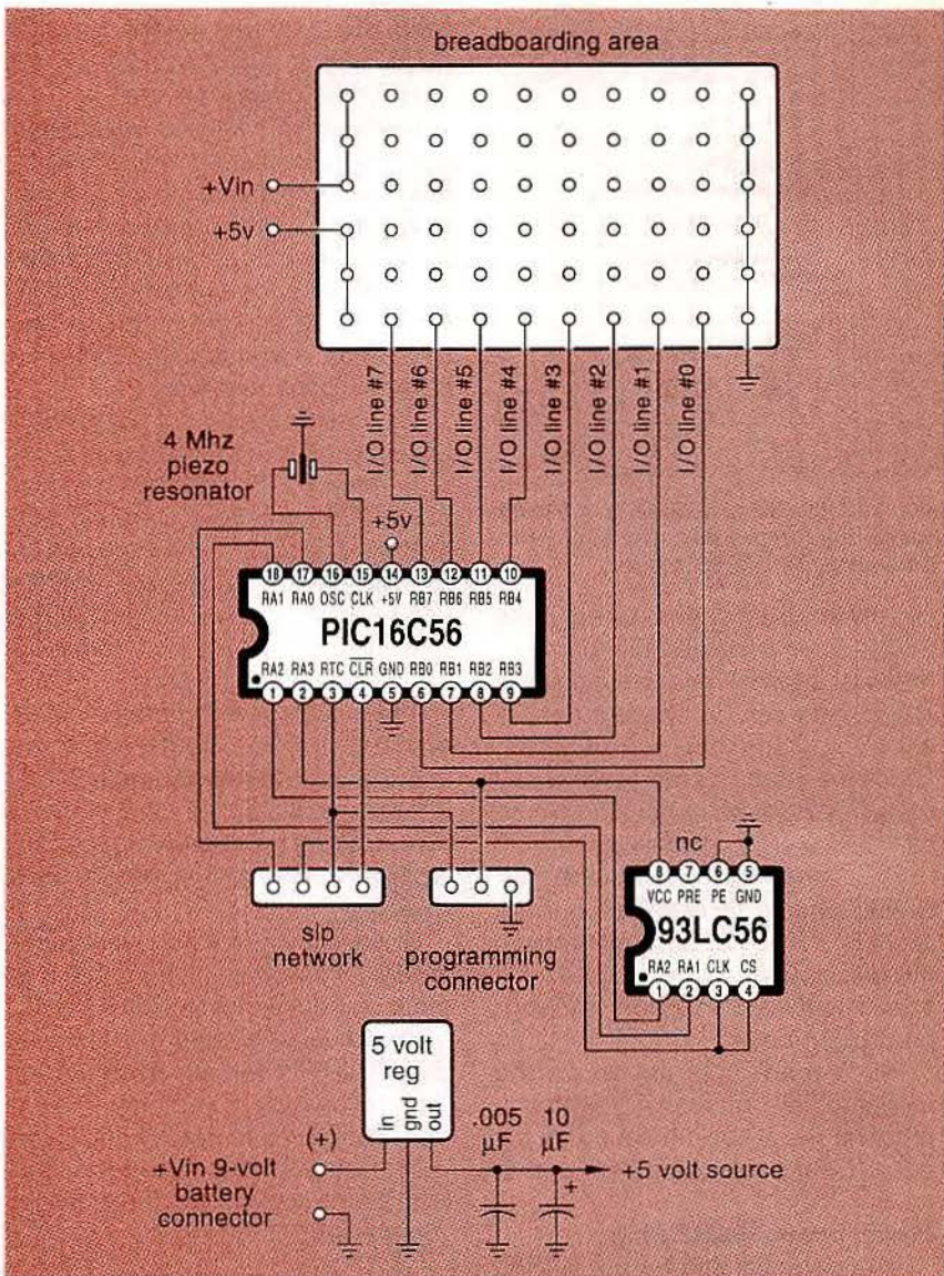
FIG. 2—SCHEMATIC DIAGRAM of the BASIC Stamp.
