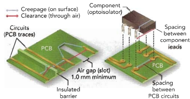
FIGURE 3. Safety standards specify creepage and clearance spacing. Artwork by Melinda Vaughan, National Instruments.
