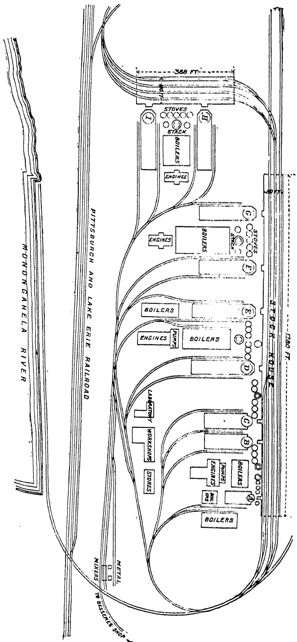
Fig. 16.—Plan of Edgar Thomson Works, Pittsburgh, Pa.
