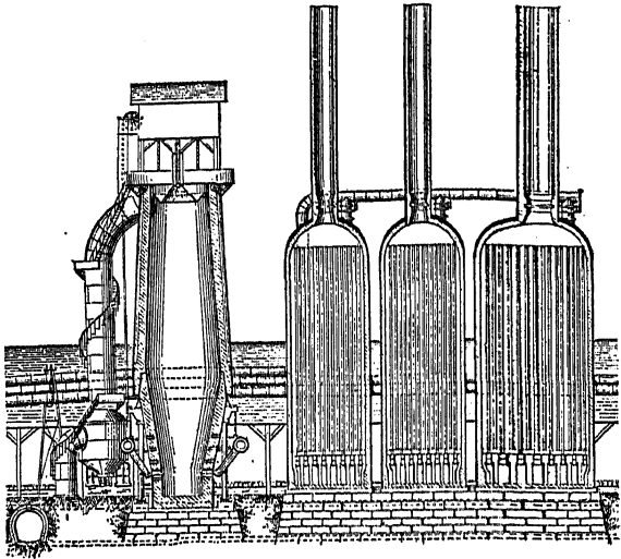
Fig. 18.—Section of blast-furnace plant, Alabama.
