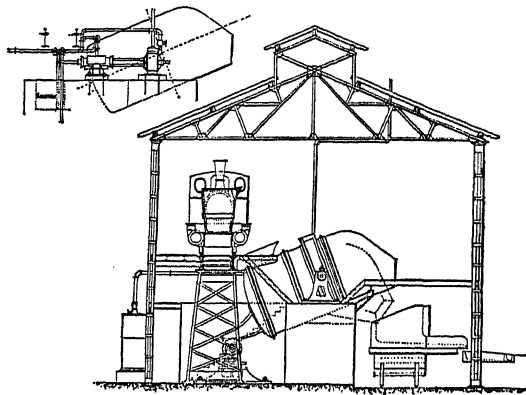
Fig. 44.—Metal mixer and desulphuriser.
