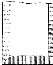
Fig. 52.—Diagram showing effect of sharp angles in a casting.
