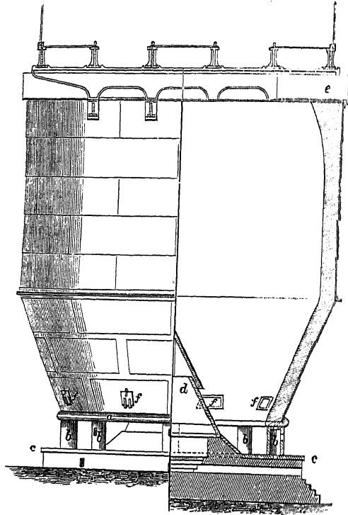
Fig. 12.—Cleveland calciner.
