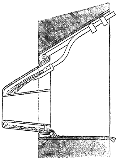
Fig. 41.—Water Cooled Open Twyer.
