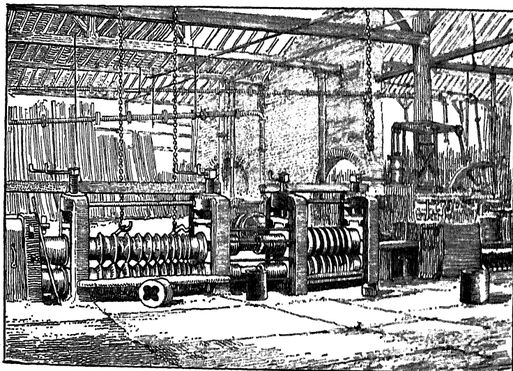
Fig. 79.—Train of two high mill rolls.
