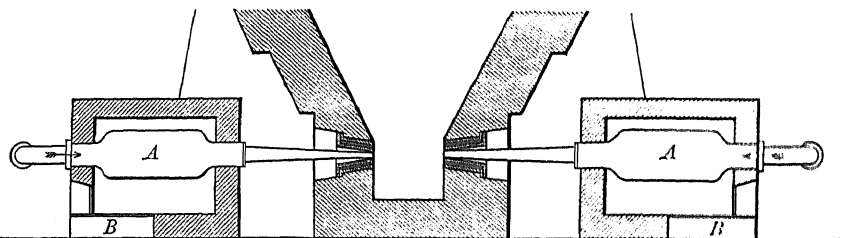
Fig. 26.—Neilson's cylindrical oven.
