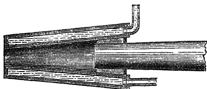
Fig. 40.—Staffordshire Twyer (Section).
