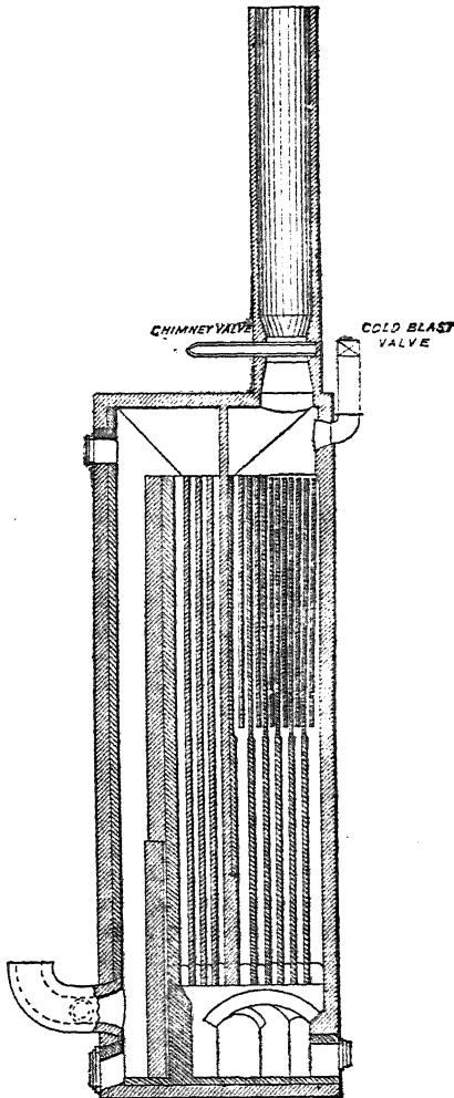
Fig. 36.—Gordon-Cowper-Whitwell stove.
