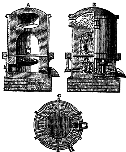
Fig. 10.—Early form of Bessemer converter.
