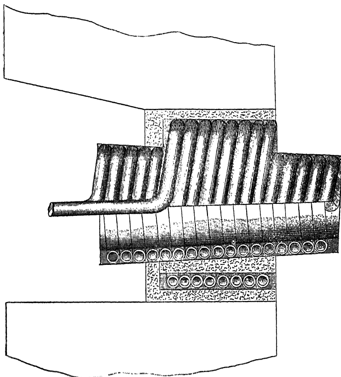
Fig. 38.—Scotch Twyer with outer coil.
