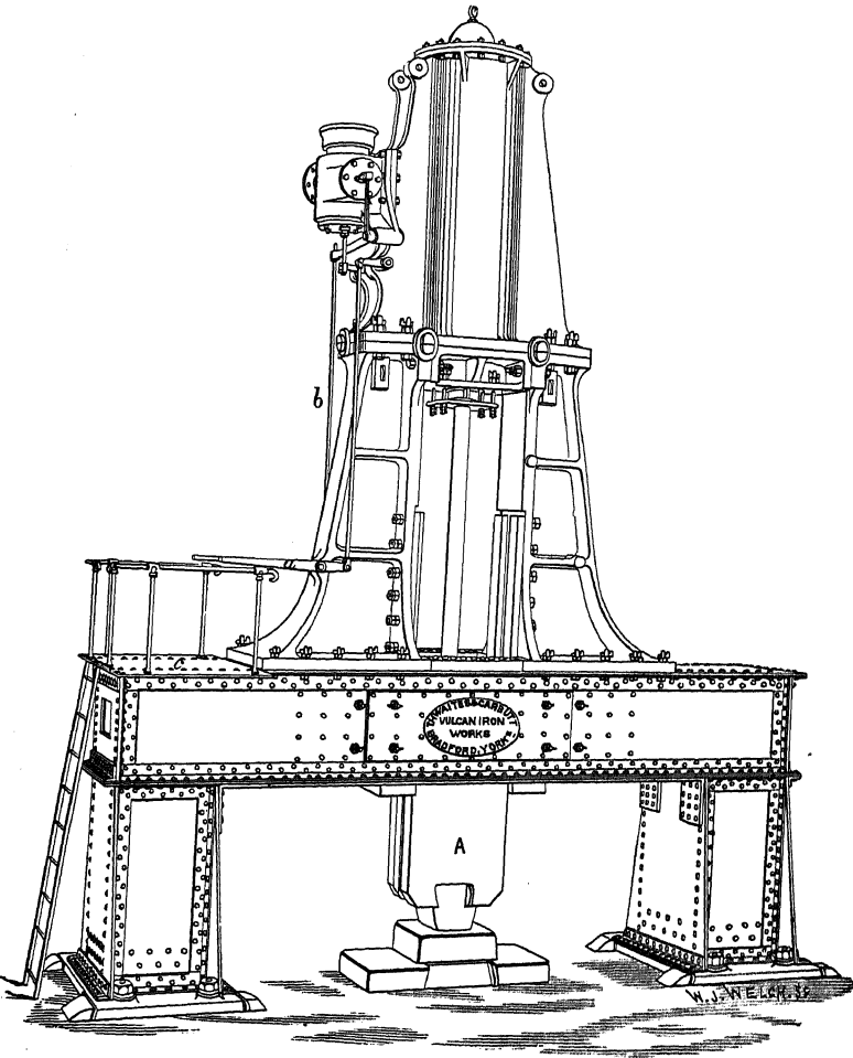
Fig. 75.—Double-acting steam hammer.
