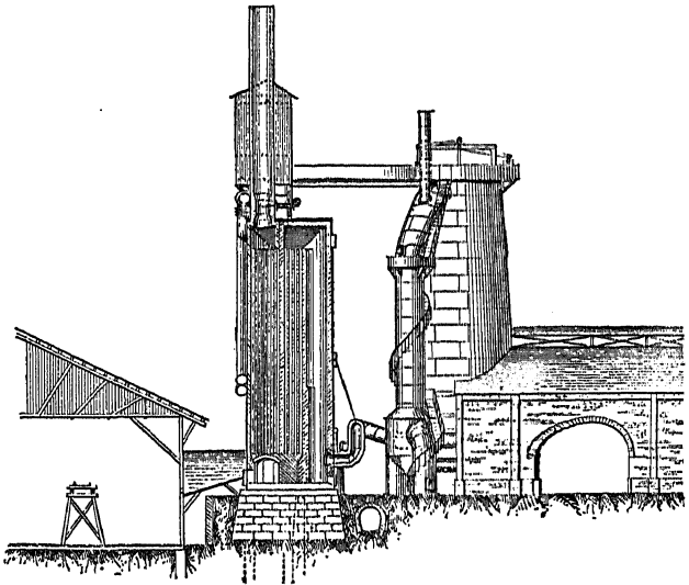
Fig. 19.—Section at right angles to Fig. 18.
