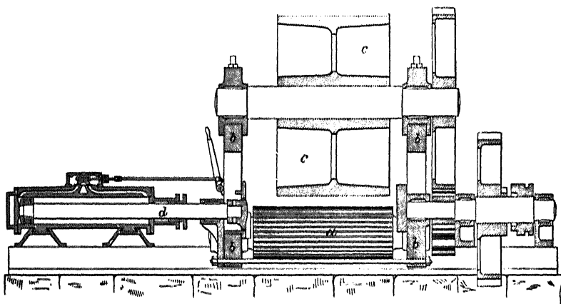
Fig. 74.—Winslow's mechanical squeezer.
