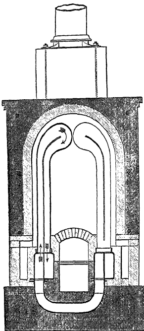
Fig. 30.—Pistol pipe stove.
