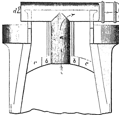
Fig. 22. - Central Tube arrangement.
