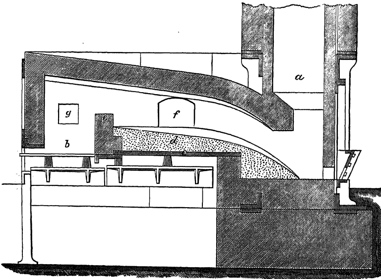
Fig. 77.—Section of mill furnace.
