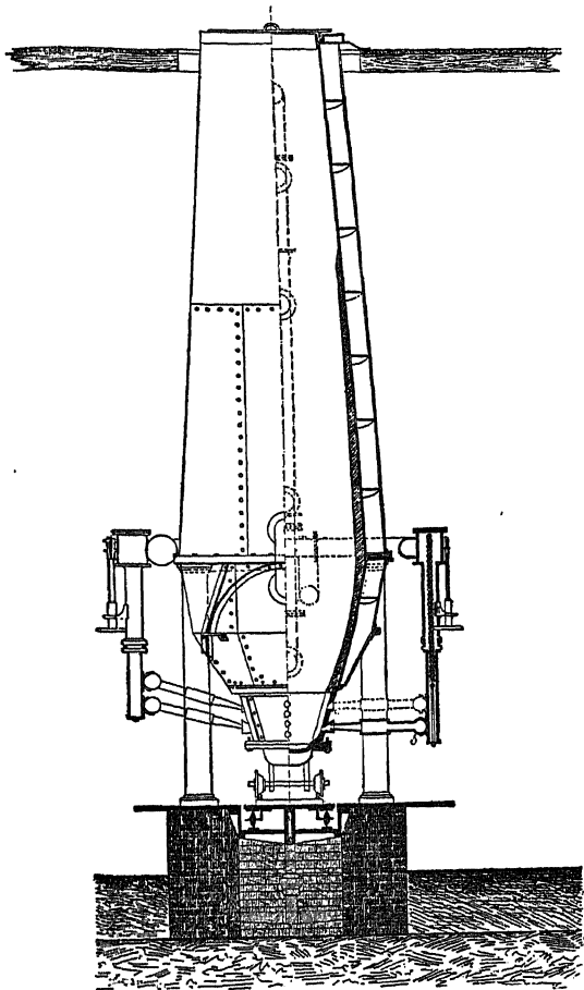
Fig. 60.—Husgafvel furnace—part section.
