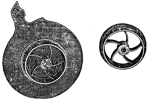
Fig. 51.—Pattern for sand moulding machine.
