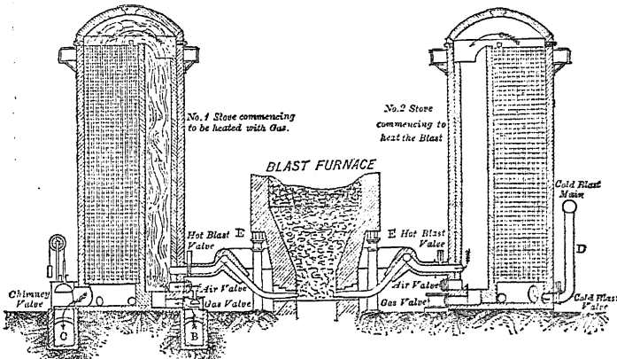
Fig. 31.—Cowper's hot-blast stoves.
