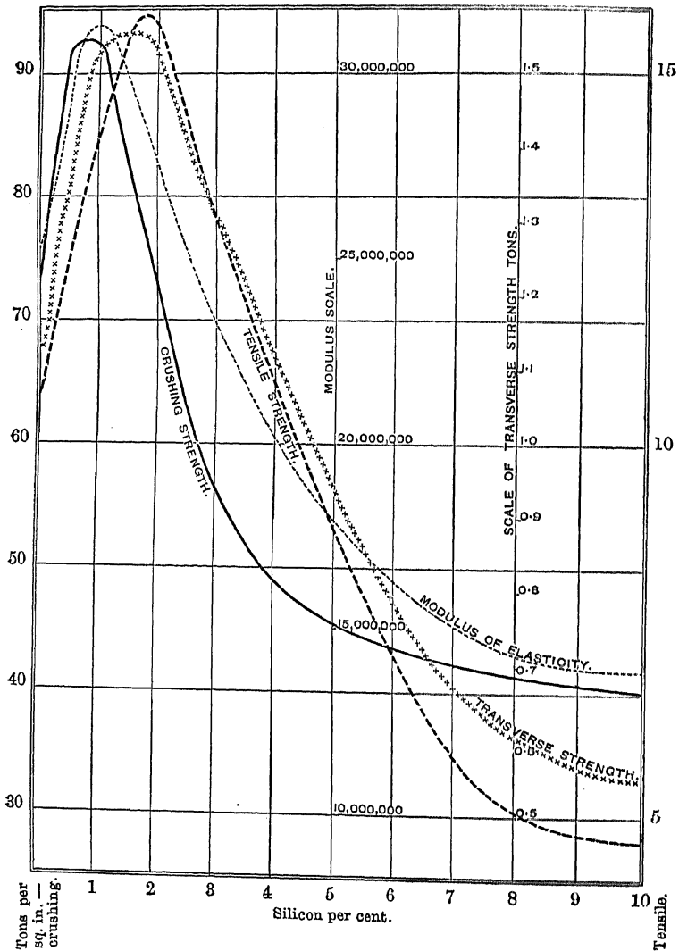
Fig. 45.—Influence of silicon on the strength of cast iron.
