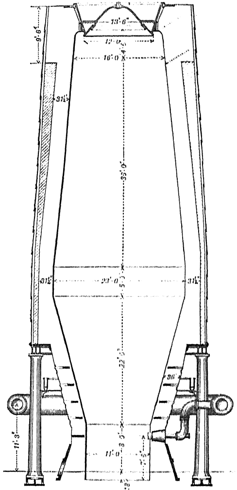
Fig. 17.—Section of blast furnace, Edgar Thomson Works.
