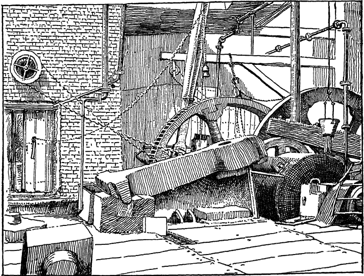
Fig. 73.—General view of Staffordshire helve.
