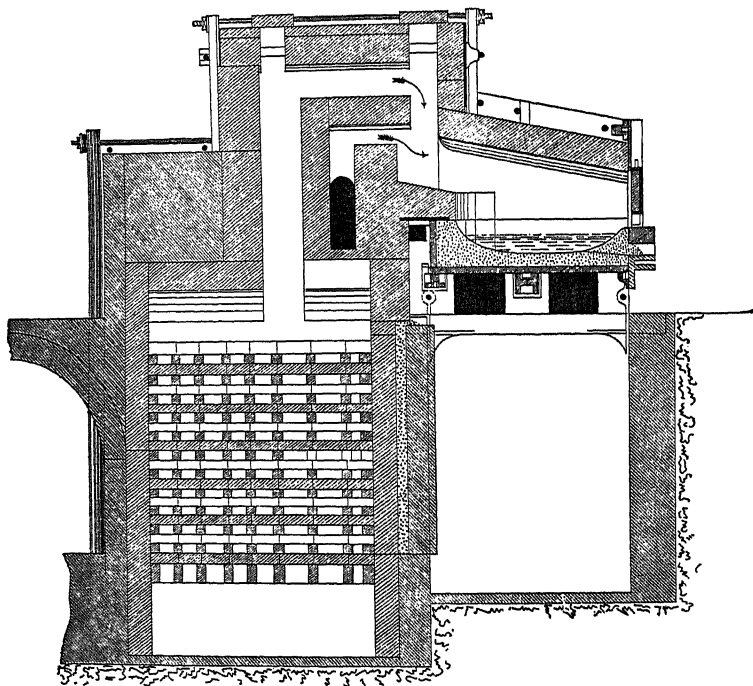
Fig. 70.—Siemens' puddling furnace.
