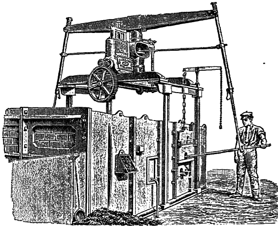
Fig. 71.—Clough's mechanical puddler.
