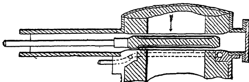
Fig. 33.—Hot-blast valve.
