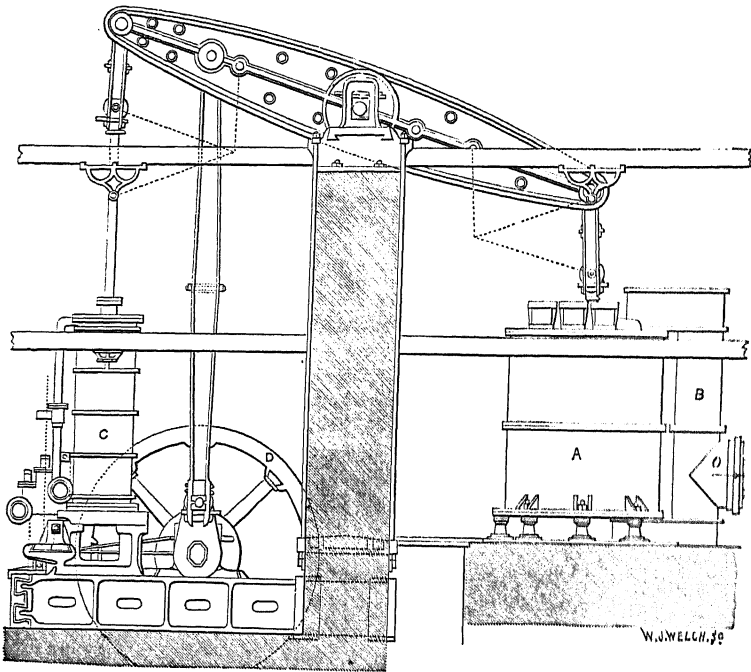
Fig. 24.—Beam Blast Engine.
