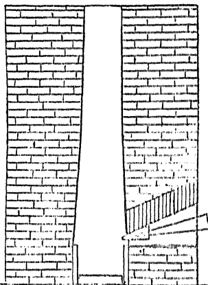
Fig. 58.—Section of the Osmund furnace.
