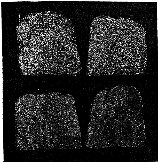
Fig. 48.—Fractures of Nos. 1, 2, 4, and white Northampton pig iron.
