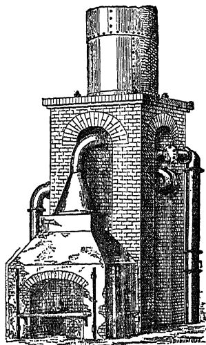
Fig. 62.—Styrian open hearth. General view.
