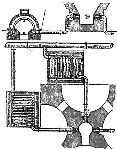
Fig. 27.—Original tubular oven.
