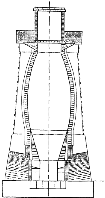
Fig. 9.—South Staffordshire blast furnace, 1860.
