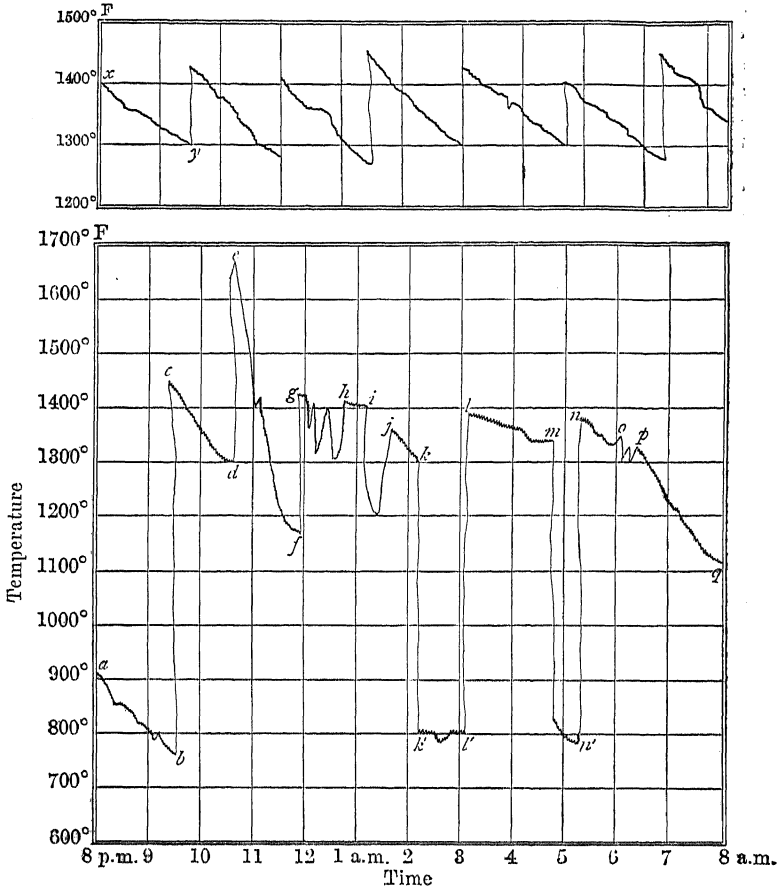
Fig. 37.—Automatic records of temperatures of hot-blast stoves.
