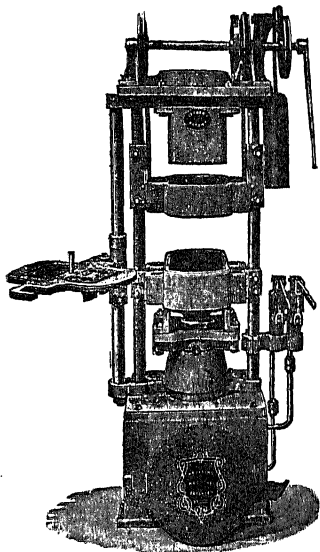
Fig. 50.—Sand moulding machine.
