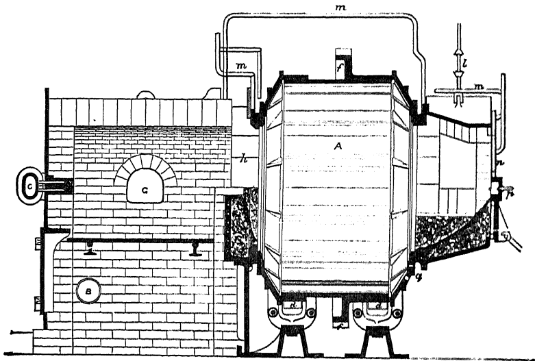
Fig. 72.—Danks' mechanical puddling furnace.
