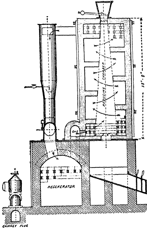
Fig. 61.—The Blair-Adams direct reduction furnace.
