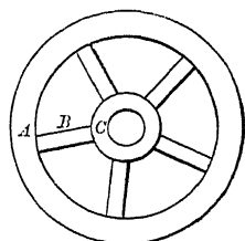
Fig. 55.—Diagram illustrating shrinkage in a cast-iron wheel.
