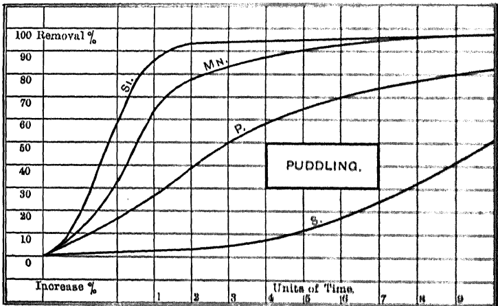
Fig. 67.—Removal of non-metals (other than carbon) in puddling.
