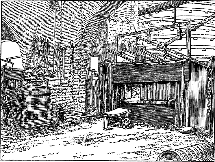
Fig. 76.—Re-heating or "mill" furnace—General view.
