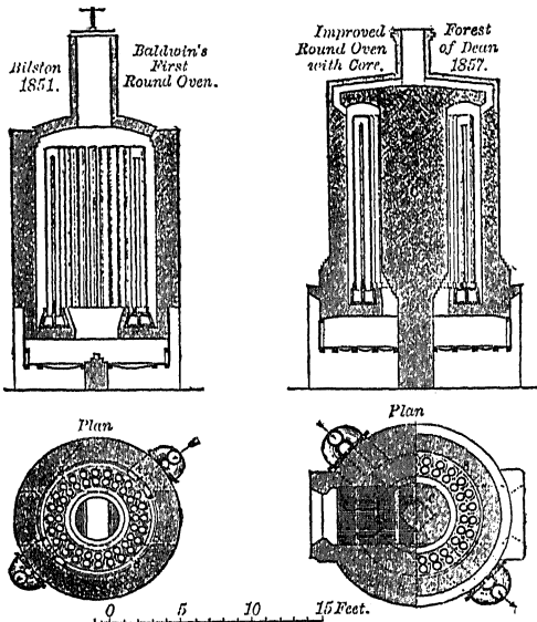
Fig. 29.—Round and long ovens.
