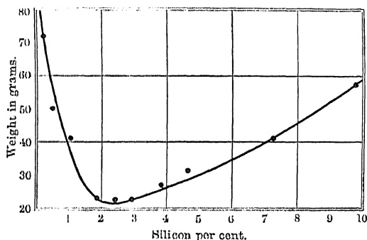
Fig. 46.—Influence of silicon on the hardness of cast iron.
