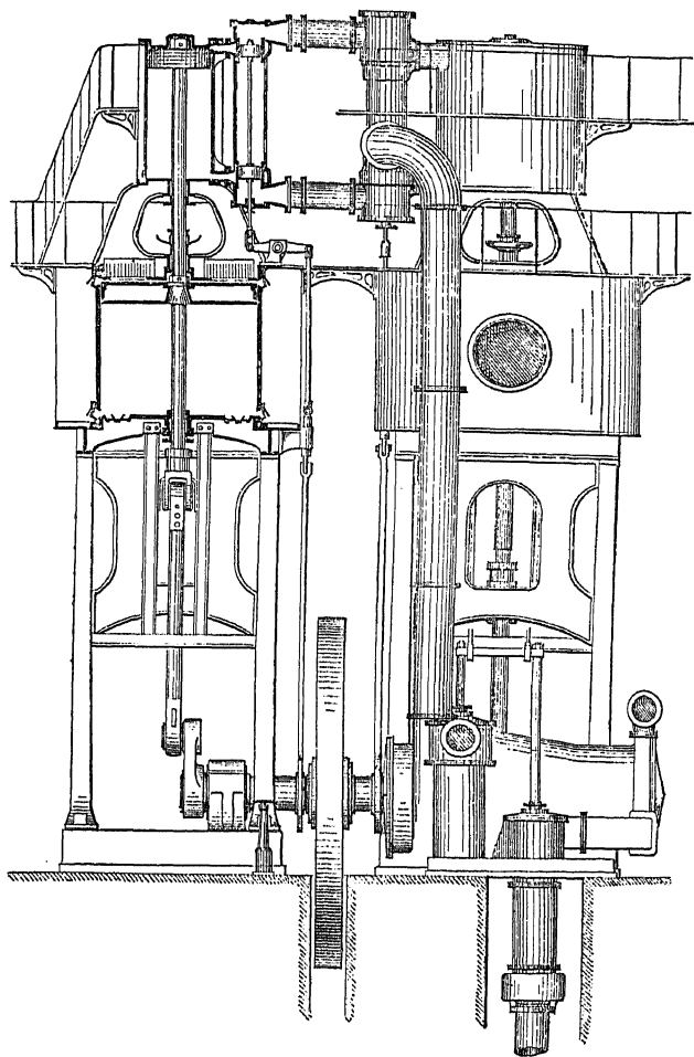
Fig. 25.—Vertical Direct-acting Blast Engine (Half Section).
