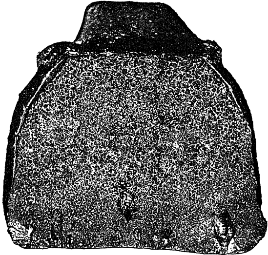
Fig. 47.—Fracture of pig iron containing titanium.
