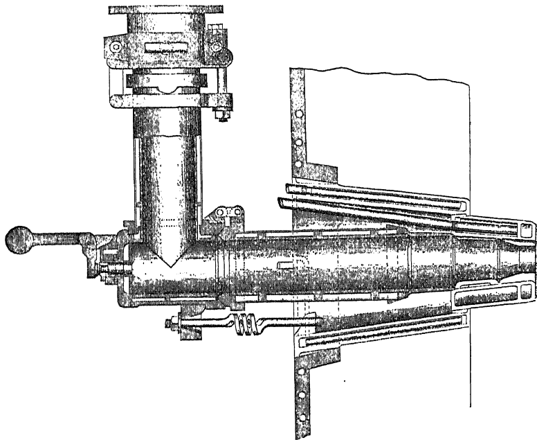
Fig. 42.—American Open Twyer.
