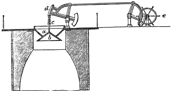
Fig. 21.—Cup and Cone arrangement.
