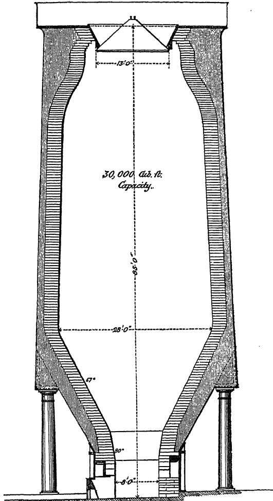
Fig. 16.—Section of Cleveland blast furnace.
