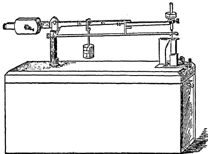
Fig. 56.—Turner's sclerometer.
