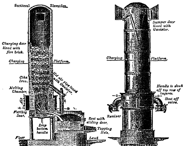
Fig. 49.—Stewart's "Rapid" cupola.
