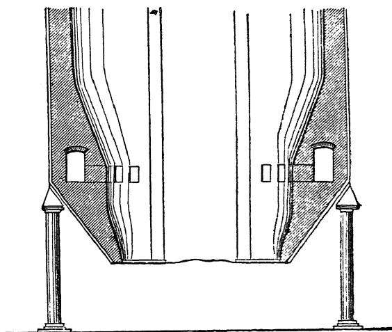
Fig. 13.—Gas-fired calciner.
