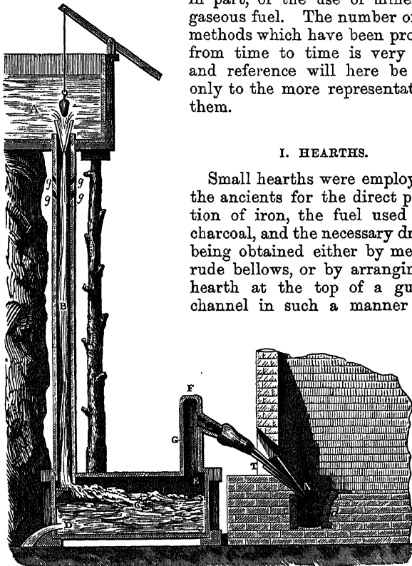
Fig. 57.—Section of Catalan forge.
