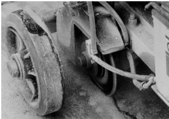
Figure 9.1. Random crack saw
