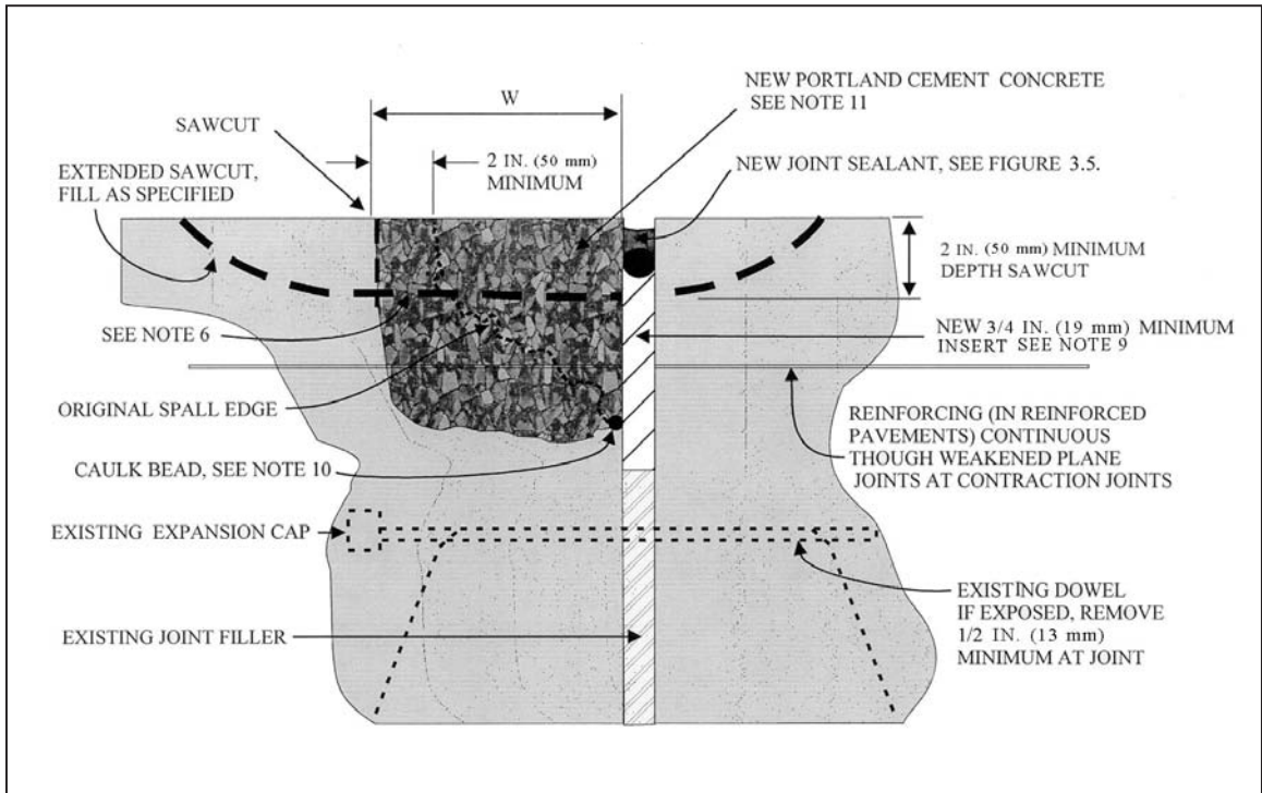
Figure 3.4. Spall repair at expansion joint
