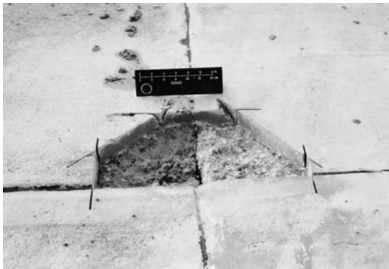
Figure 15.1. A spalled area on both sides of an expansion joint ready for installation of joint filler
