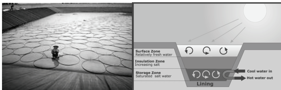
Fig. 2a. (Left) Solar pond for heating purpose demonstration in Australia ( http://www.aph.gov.au/library/pubs/bn/sci/RenewableEnergy_4.jpg ). 2b. (Right) Solar Ponds Schematic The salt content of the pond increases from top to bottom. Water in the storage zone is extremely salty. As solar radiation is absorbed the water in the gradient zone cannot rise, because the surface-zone water above it contains less salt and therefore is less dense. Similarly, cooler water cannot sink, because the water below it has a higher salt content and is denser. Hot water in the storage zone is piped to, for example, a boiler where it is heated further to produce steam, which drives a turbine. (Wright, 1982; and www.energyeducation.tx.gov/.../index.html )
