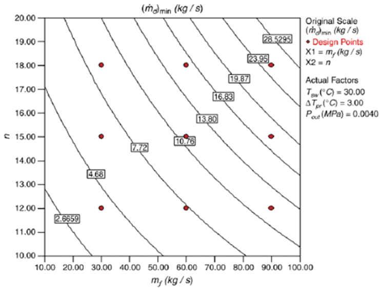
Fig. 6. Contour of minimum distilled water for T_{sw}=30^\circ\text{C} , \Delta T_{pr}=3^\circ\text{C} , P_{out}=0.004\text{MPa}
