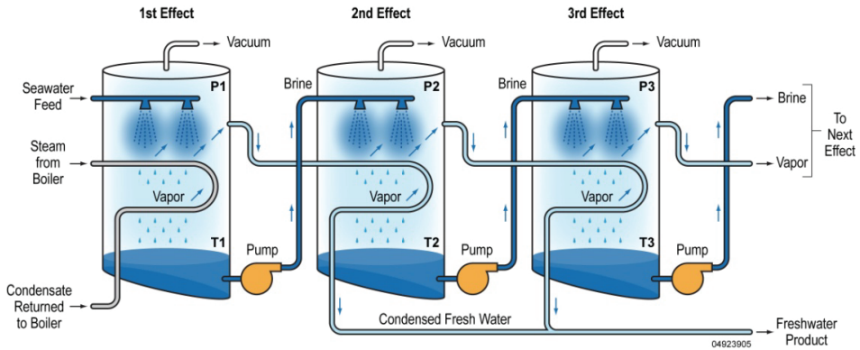
Fig. 5. Diagram of an MED unit (modified from [7])
