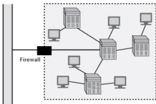
Exhibit 10.: An Intranet
