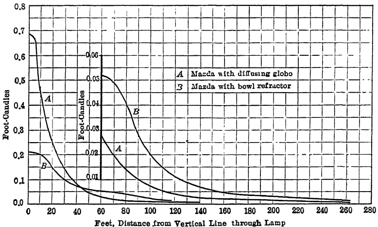
Fig. 100.—Results of illumination calculations.
