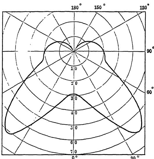
FIG. 62.—Distribution curve for Holophane reflector XE-40, with 40-watt lamp.
