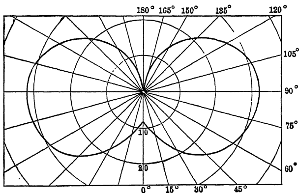
FIG. 78.—Distribution curve for 40-watt, clear-tip, tungsten lamp, bare.
