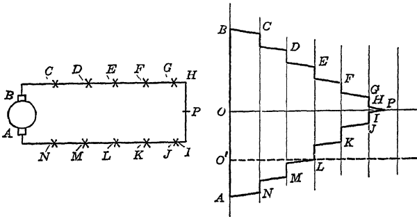
FIG. 11.—Series circuit and its potential gradient.
