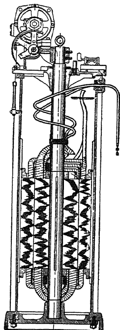
FIG. 17.—Motor-operated induction type of potential regulator.
