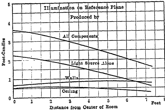
FIG. 77.—Various components of total illumination upon reference plane.
