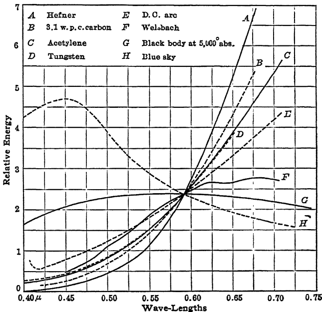
FIG. 51.—Spectrophotometric curves for different light-sources.
