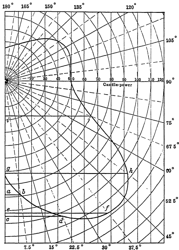
FIG. 56.—Flux-o'-lite paper.
