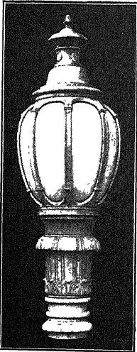
FIGS. 91 and 92.—Ornamental type luminous arc with diffusing glass globe and distribution curves for: (A) 6.6-ampere, long-life electrode, and medium diffusing glass. (B) 5-ampere, high-efficiency electrode, and medium diffusing glass. (C) 5-ampere, long-life electrode, and medium diffusing glass. (D) 4-ampere, high-efficiency electrode, and medium diffusing glass. (E) 4-ampere, long-life electrode, and medium diffusing glass.
