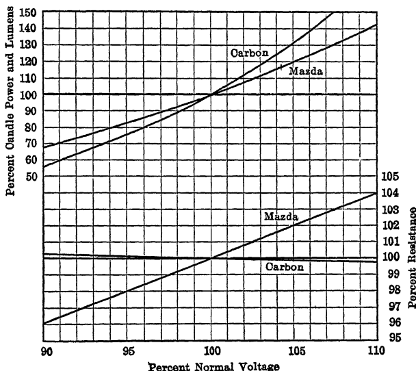
FIG. 26.—Percentage variations in candle-power, lumens and resistance with variation in voltage of operation of incandescent lamps.
