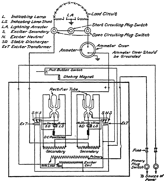
FIG. 20.—Diagram of circuits for two-tube mercury-arc rectifier.
