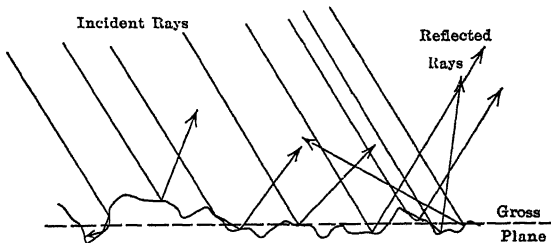
FIG. 36.—Diffusion of light by reflection.
