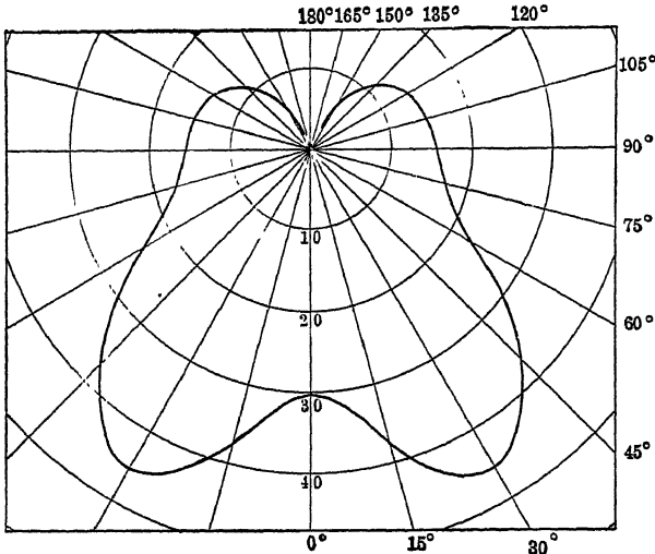
FIG. 79.—Distribution curve for 40-watt, frosted tip, tungsten lamp, with prismatic reflector.
