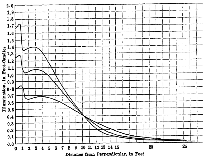
FIG. 75.—Intensity of illumination of working plane by one 75-watt lamp fitted with a reflector having a velvet finish, for different elevations.
