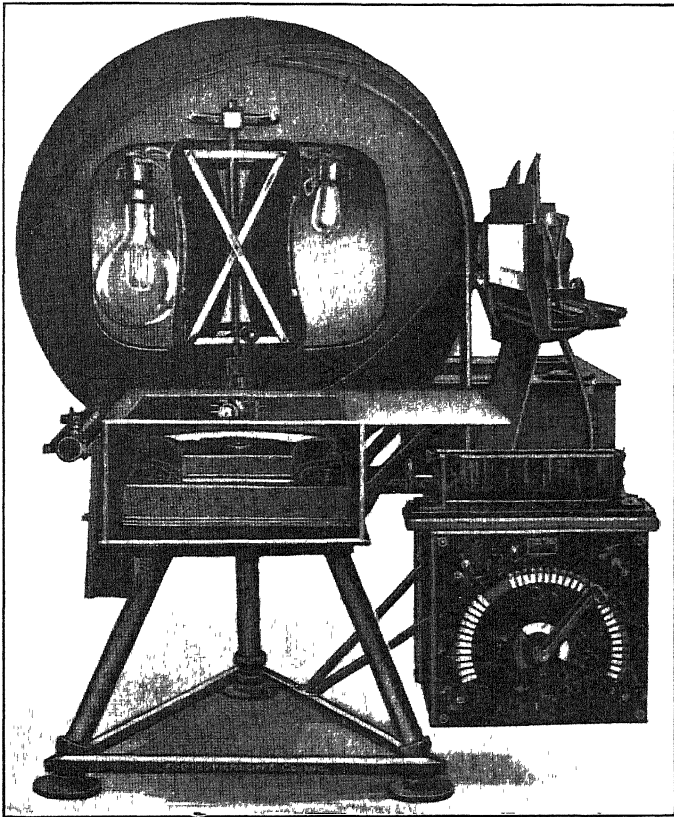
FIG. 47.—Globe photometer and accessories.
