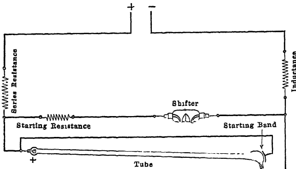
Fig. 31.—Diagram of circuits of mercury-vapor lamp.
