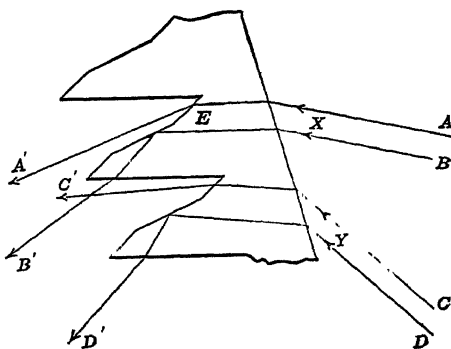
FIG. 68.—Principle of prismatic globes and shades—outer surface.
