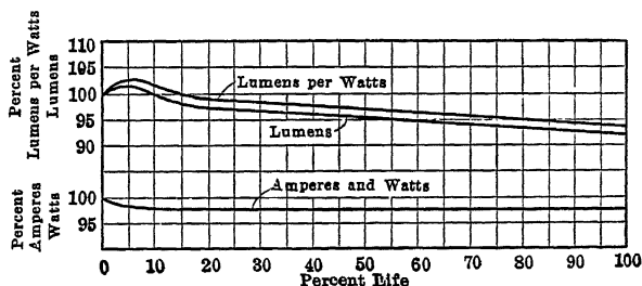
FIG. 25.—Typical performance curves of Mazda type-C lamps.
