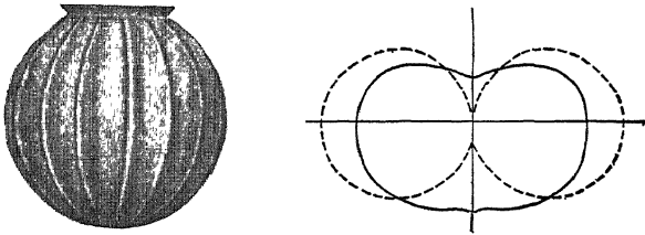
FIG. 70.—Opal bowl and distribution curve.
