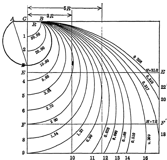
FIG. 59.—Equilux spheres.
