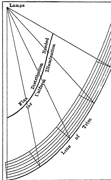
FIG. 83. To find light flux distribution needed for uniform illumination of given store window.
