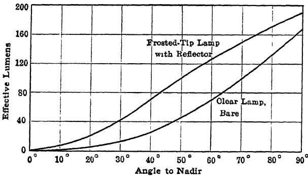
FIG. 80.—Effective lumens for various angles below 40-watt, tungsten lamps.
