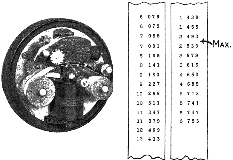
FIG. 21.—Type P demand indicator (Printometer, General Electric Co.), with record.
