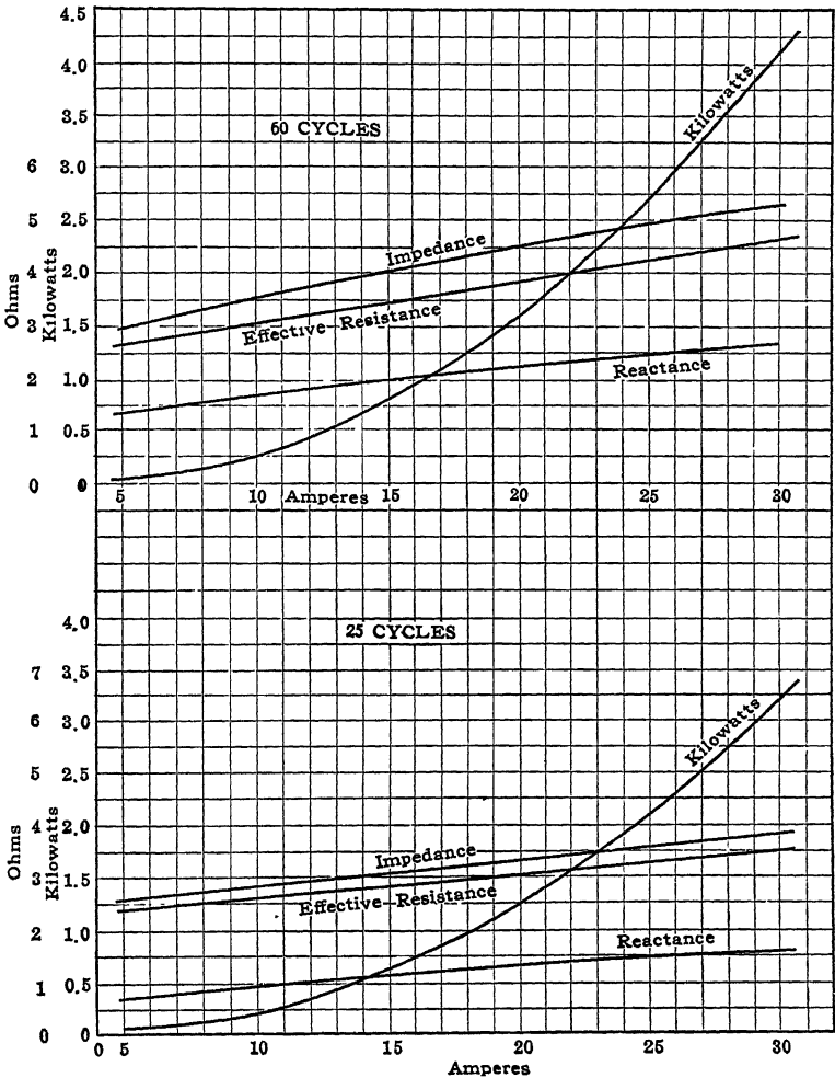
FIG. 3.—Constants for one mile of \frac{1}{2} -inch galvanized stranded steel cable at 25 cycles and 60 cycles per second. Direct-current resistance per mile of cable is 2.42 ohms.
