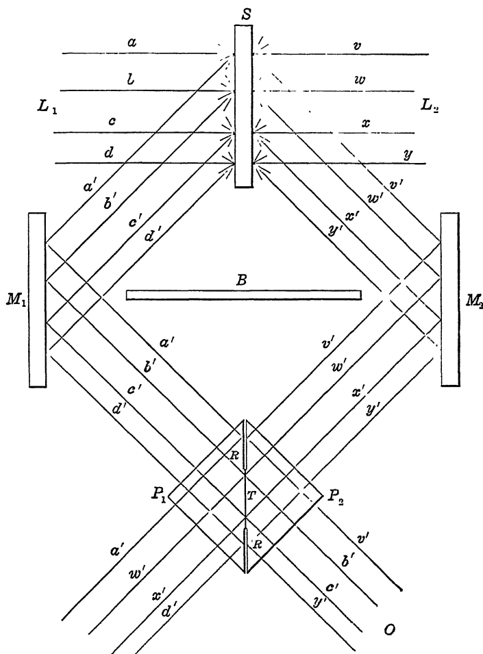
FIG. 44.—Lummer-Brodhun sight box.
