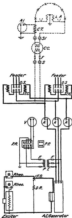
FIG. 14.—Diagram of circuits for separately excited, 3-phase arclight generator, with two sets of feeders at constant potential and one arc circuit.
