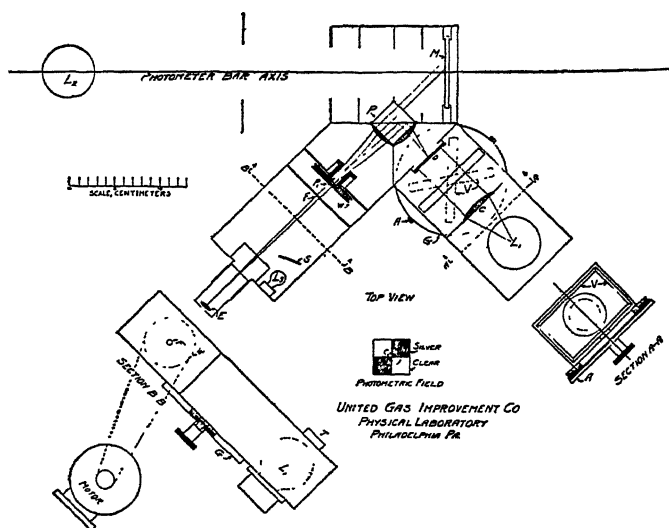
FIG. 48.—Flicker photometer.
