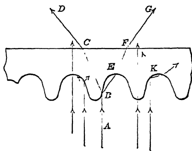
FIG. 67.—Principle of prismatic globes and shades—inner surface.
