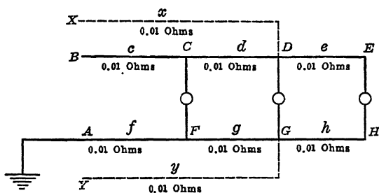
FIG. 13.—Simple parallel circuit without and with feeders.
