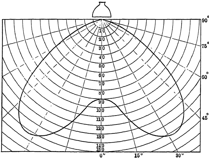
FIG. 55.—Vertical distribution curve, X-ray reflector No. 555.
