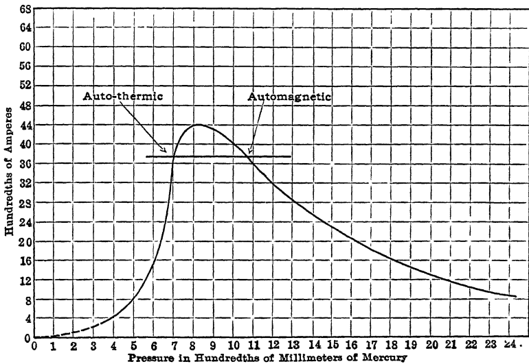
FIG. 30.—Characteristics of Moore tube.
