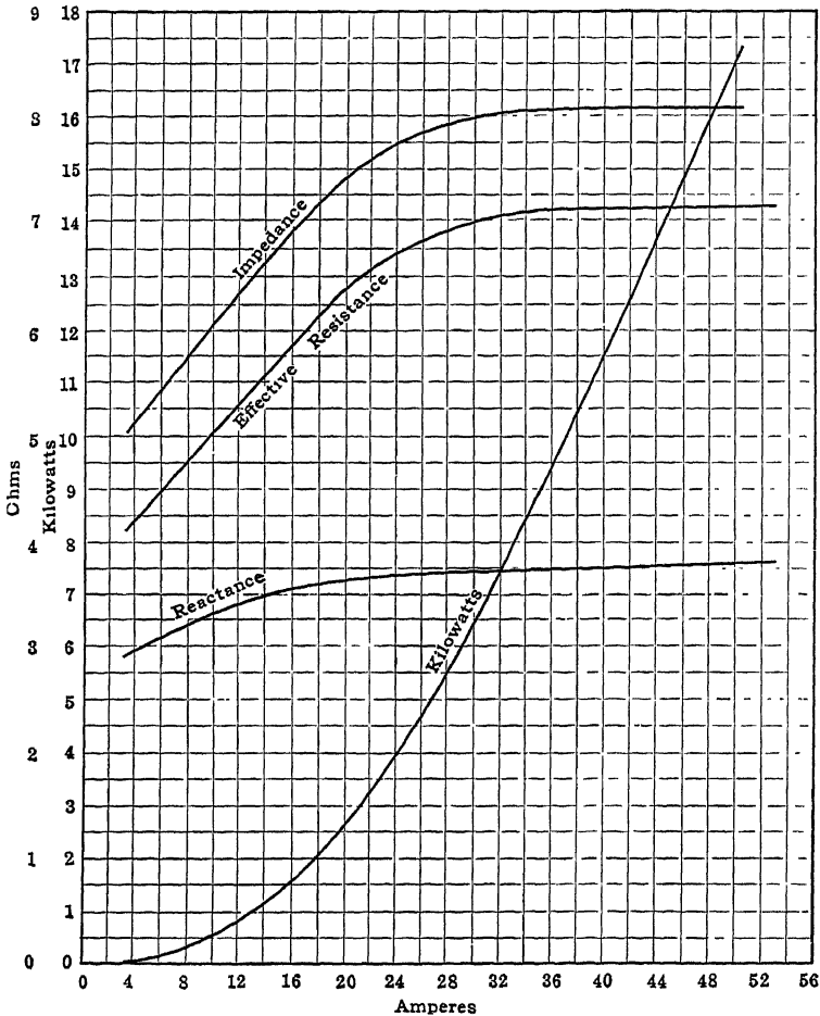
FIG. 6.—Constants for one mile of \frac{3}{8} -inch galvanized stranded EBB iron cable at 60 cycles per second. Direct-current resistance per mile of cable is 3.6 ohms. Tests made on three-phase circuit with wires in one plane on 24-inch centers.
