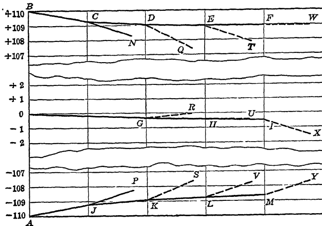
FIG. 12.—Parallel circuit and its potential gradient.
