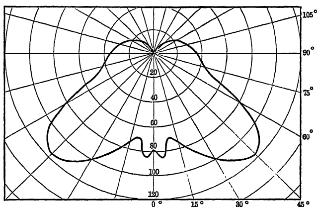
FIG. 74.—Distribution curve for 75-watt Mazda lamp with reflector.
