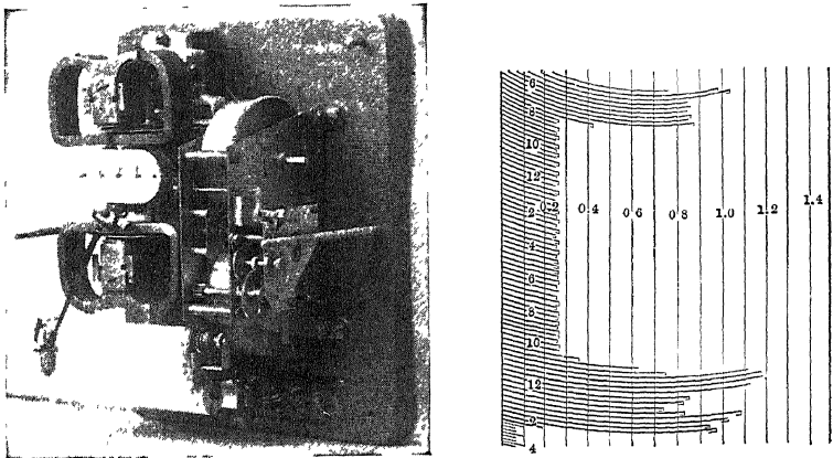
FIG. 22.—Recording-demand watt-hour meter; Westinghouse, type RA, with record.
