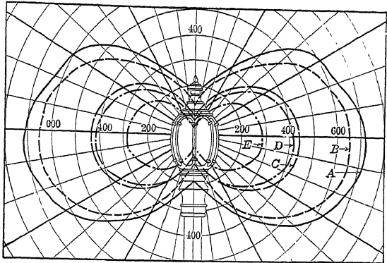
FIGS. 91 and 92.—Ornamental type luminous arc with diffusing glass globe and distribution curves for: (A) 6.6-ampere, long-life electrode, and medium diffusing glass. (B) 5-ampere, high-efficiency electrode, and medium diffusing glass. (C) 5-ampere, long-life electrode, and medium diffusing glass. (D) 4-ampere, high-efficiency electrode, and medium diffusing glass. (E) 4-ampere, long-life electrode, and medium diffusing glass.
