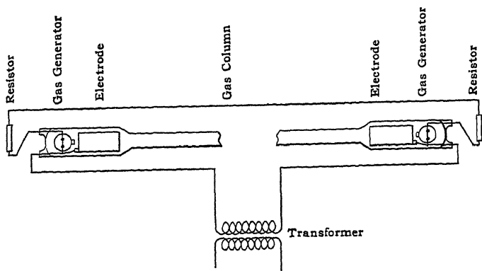
FIG. 29.—Diagram of circuits of Moore tube.
