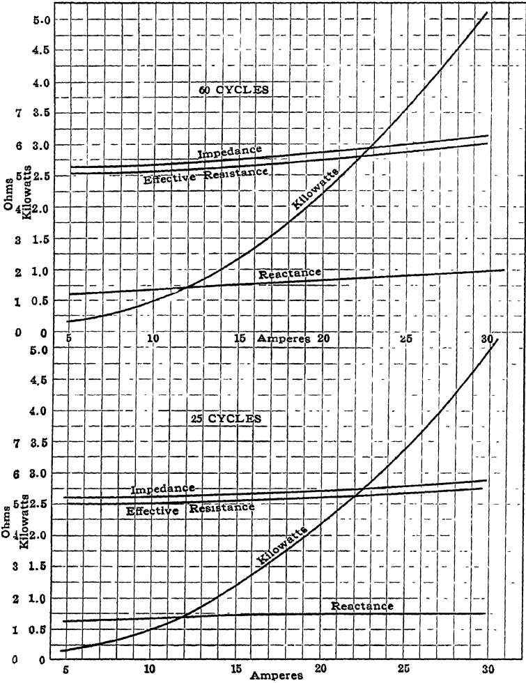
FIG. 2.—Constants for one mile of \frac{3}{8} -inch galvanized stranded steel cable at 25 cycles and 60 cycles per second. Direct-current resistance per mile of cable is 5.03 ohms.
