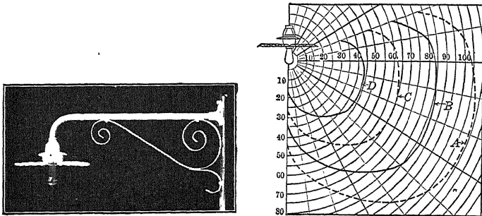
FIGS. 94 and 95.—Mazda series lamp with flat radial-wave reflector, and distribution curves for: (A) 100-c.-p. mazda. (B) 80-c.-p. mazda. (C) 60-c.-p. mazda. (D) 40-c.-p. mazda.
