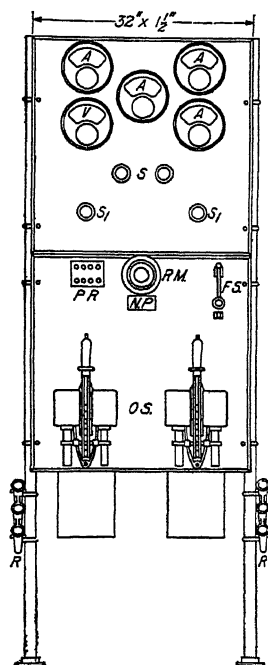
FIG. 15.—Switchboard panel for 2300-volt, 3-phase generator with two sets of feeders at constant potential, and one arc circuit.
