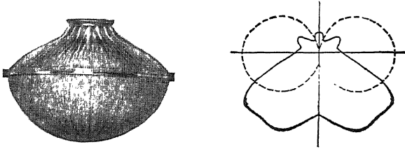
FIG. 69.—Twelve-inch prismatic reflection-bowl and distribution curve.
