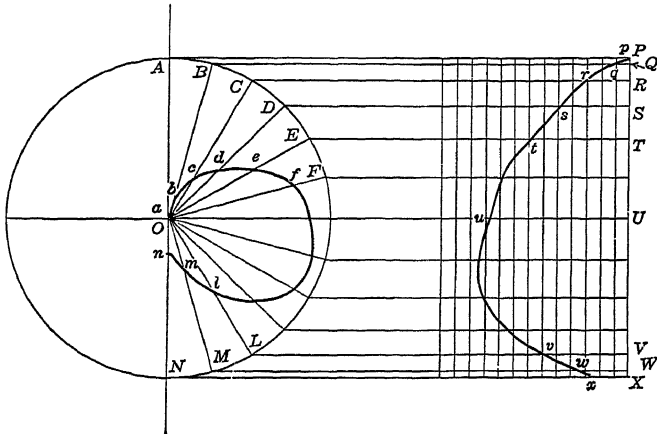
FIG. 57.—Elementary Rousseau diagram.
