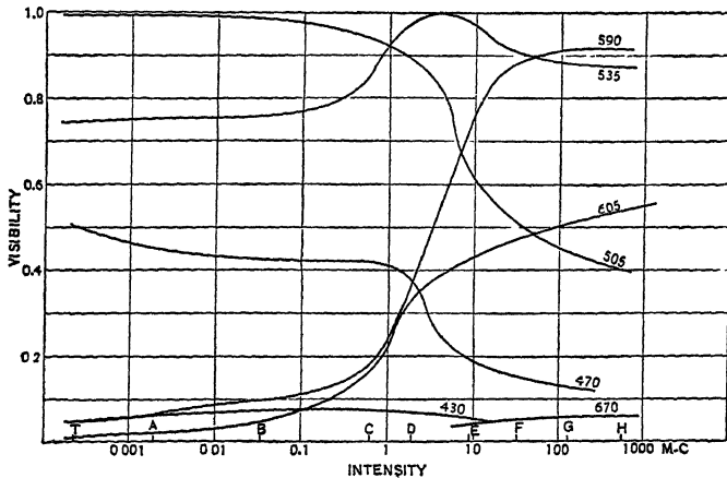
FIG. 38.—Relative visibility curves of various colors of light, as a function of intensity of illumination.
