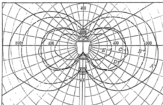
FIGS. 89 and 90.—Ornamental type luminous arc lamp and distribution curve for electrodes and diffusing glass globes as follows: (A) 6.6-ampere, long-life; medium density glass. (B) 5-ampere, high efficiency; medium density glass. (C) 5 ampere, long-life; light density glass. (D) 4-ampere, high-efficiency; light density glass. (E) 4-ampere, long-life; light density glass.
