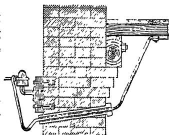
FIG. 7.—A simple, low-voltage entrance.
