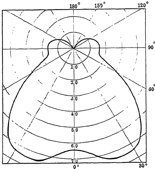
FIG. 64.—Distribution curve for Holophane reflector XI-40, with 40-watt lamp.
