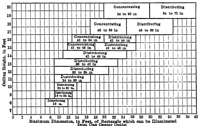
FIG. 82.—Type of reflector and length of suspension for indirect lighting system.
