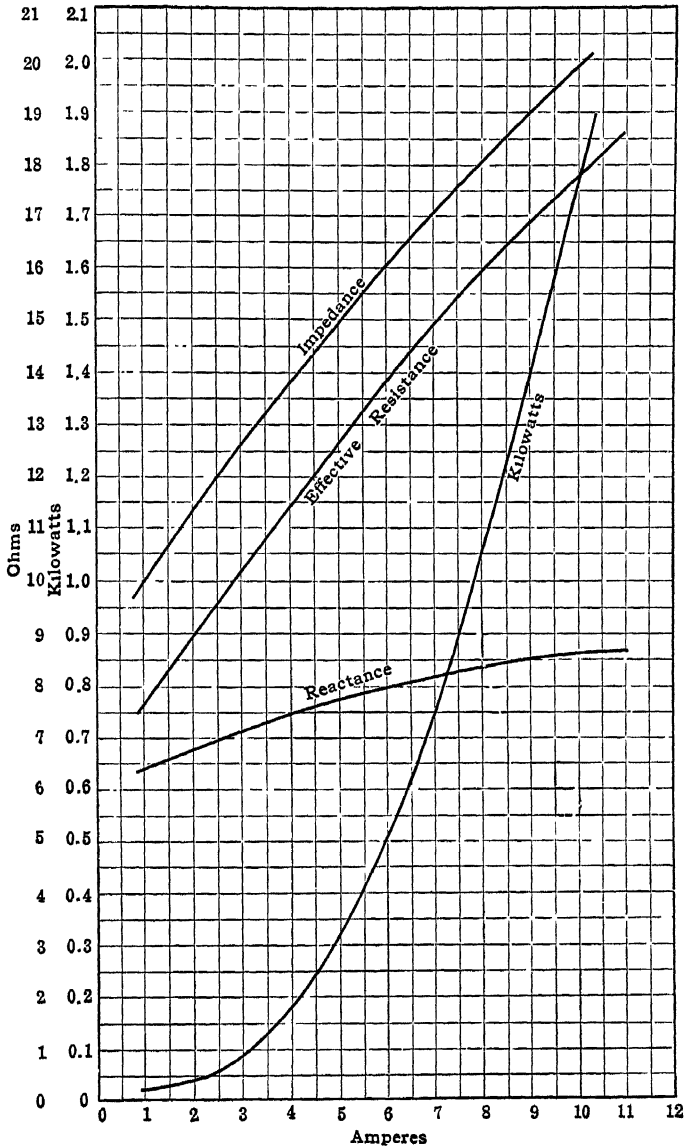
FIG. 5.—Constants for one mile of No. 4 B.W.G. solid EBB galvanized iron wire at 60 cycles per second. Direct-current resistance per mile of wire is 5.97 ohms. Tests made on three-phase circuit with wires in one plane on 42-inch centers.
