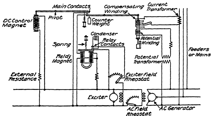
FIG. 18.—Simple diagram of circuits for automatic potential regulator.
