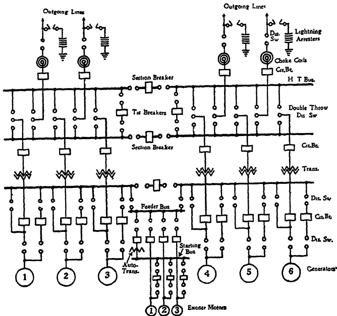
FIG. 16.—Operating features of circuits.
