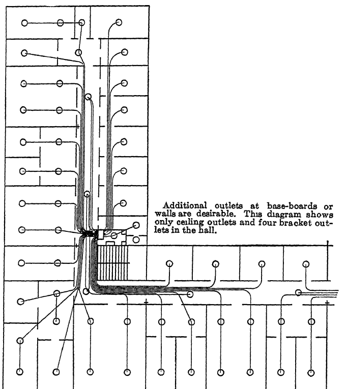
FIG. 10.—Conduit system for electric wiring for one floor of an office building.
