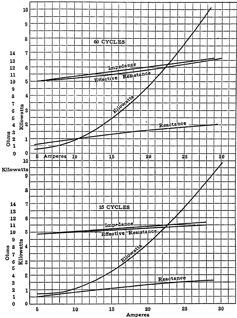
FIG. 1.—Constants for one mile of \frac{1}{4} -inch galvanized stranded steel cable at 25 cycles and 60 cycles per second. Direct-current resistance per mile of cable is 9.72 ohms.
