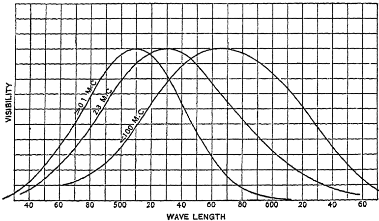
FIG. 39.—Relative visibility curves for various intensities of light, as a function of wave lengths.
