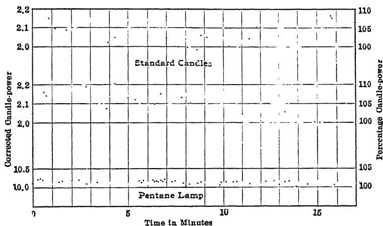
FIG. 40.—Flame-intensity variations for standard candles and pentane lamp.
