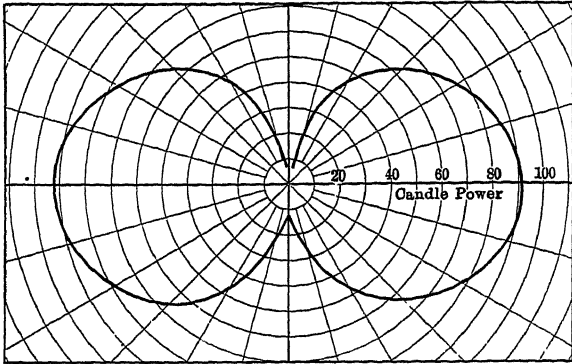
FIG. 23.—Vertical distribution curve of light flux from incandescent lamp.
