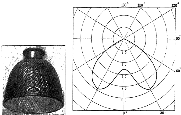
FIG. 61.—X-ray reflector, No. 555 and its distribution curve with 40-watt lamp.
