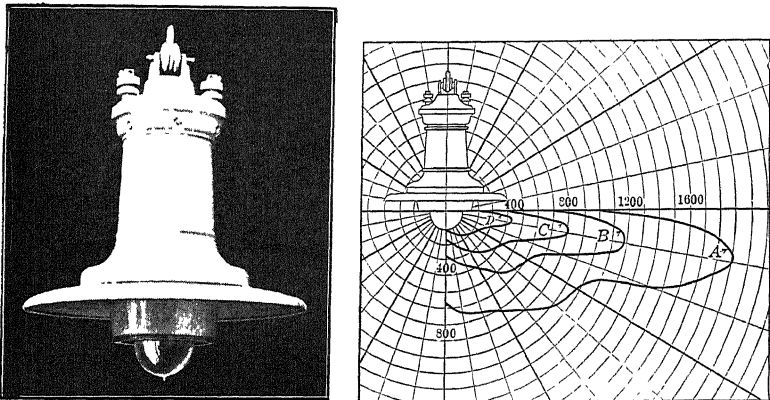
FIGS. 96 and 97.—Novalux pendant unit, steel reflector and prismatic glass band refractor and distribution curves for: (A) 1000-c.-p., 20-ampere mazda series lamp. (B) 600-c.-p., 20-ampere, mazda series lamp. (C) 400-c.-p., 15-ampere, mazda series lamp. (D) 250-c.-p., 6.6-ampere, mazda series lamp.
