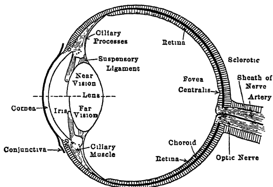
FIG. 32.—The human eye.
