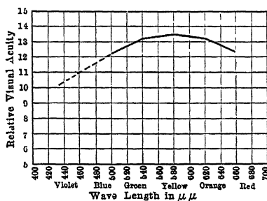
FIG. 37.—Relative visual acuity for different wave lengths.
