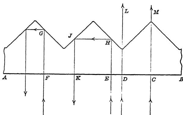
FIG. 63.—Principle of prismatic reflector.
