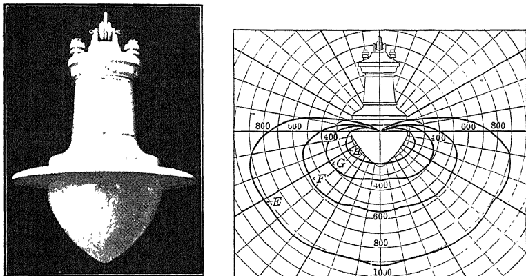
FIGS. 98 and 99.—Steel reflector and diffusing glass globe and distribution curves for: (E) 1000-c.-p., 20-ampere, mazda series lamp. (F) 600-c.-p., 20-ampere, mazda series lamp. (G) 400-c.-p., 15-ampere, mazda series lamp. (H) 250-c.-p., 6.6-ampere, mazda series lamp.
