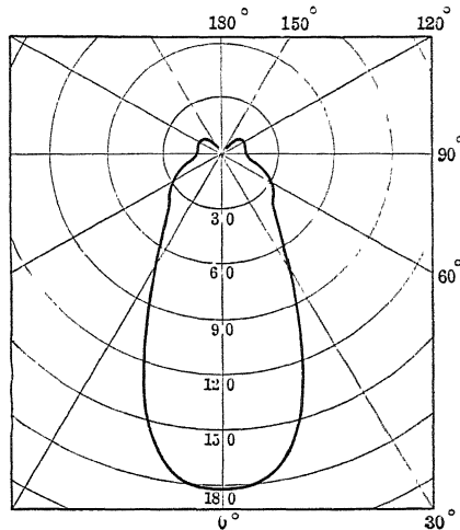
FIG. 65.—Distribution curve for Holophane reflector XF-40, with 40-watt lamp.
