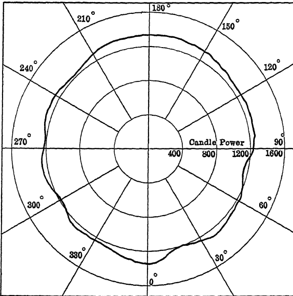
FIG. 24.—Equatorial light flux from 750-watt, 1000-c.-p., nitrogen-filled tungsten-filament lamp.
