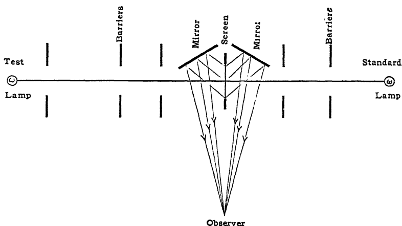
FIG. 43.—Bunsen photometer.
