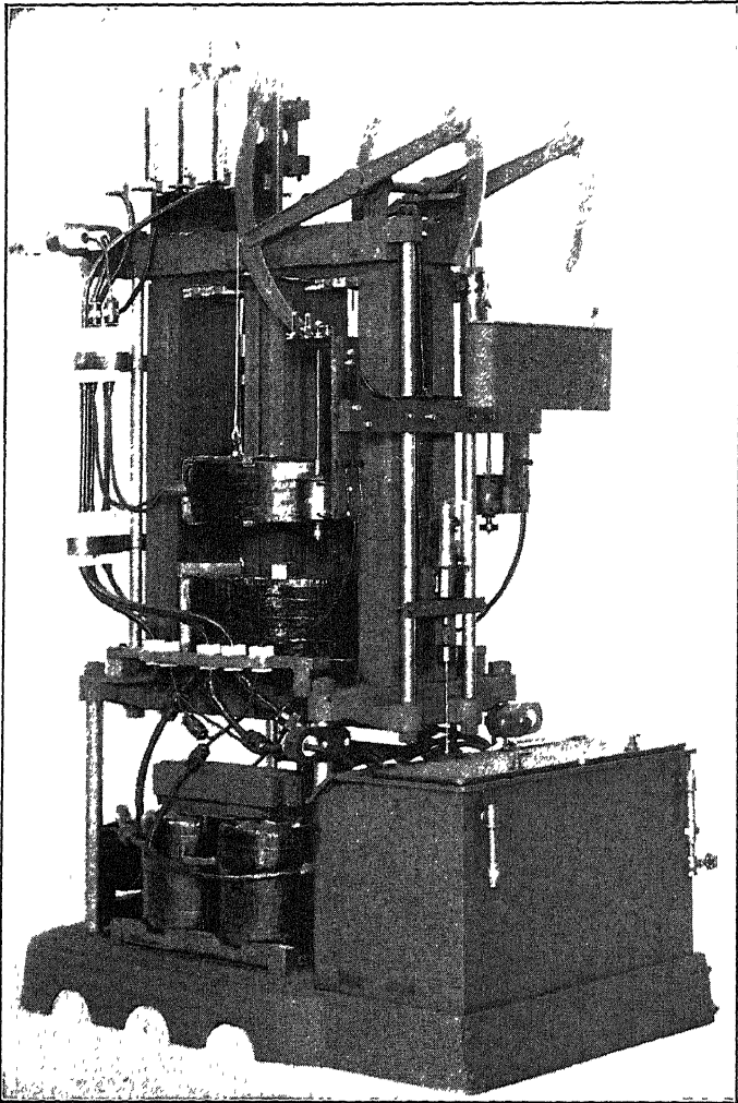
FIG. 19.—Constant-current transformer with double-tube mercury-arc rectifier; General Electric, 6600–6750 volts, 75 lights.
