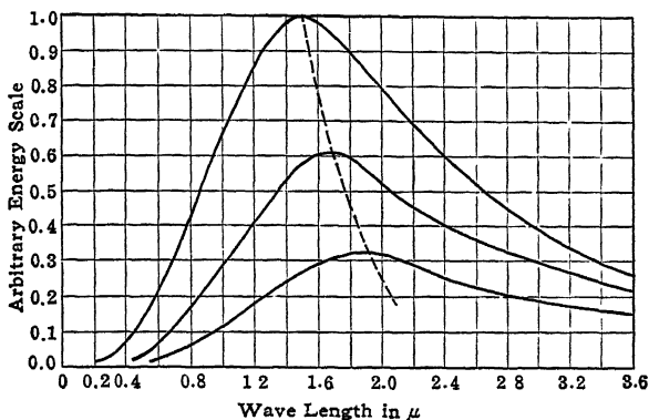
FIG. 34.—Radiation from carbon filament at different temperatures, showing shift of maximum point.
