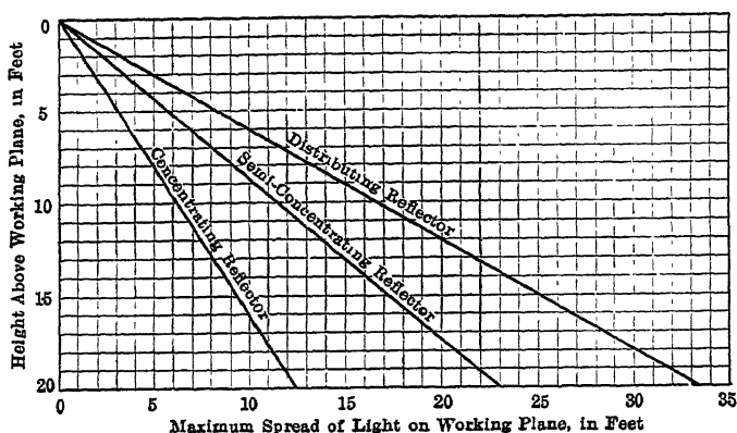
FIG. 81.—Spread of light with direct lighting system.
