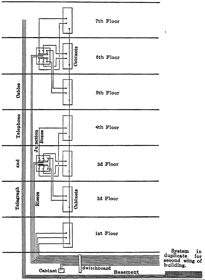
FIG. 9.—Systems of feeders and risers for an office building.
