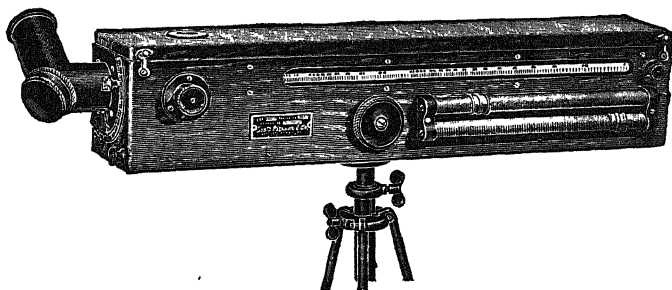
FIG. 49.—Sharp-Millar universal photometer, Model F2410, standard size.
