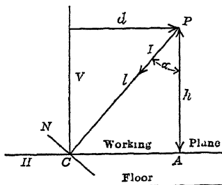
FIG. 72.—Point-by-point calculations of illumination.
