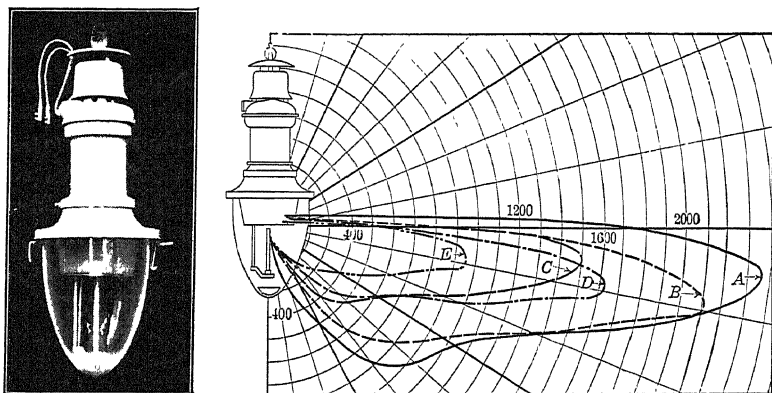
Figs. 86 and 87.—Pendant type of luminous arc lamp with prismatic refractor and distribution curves for electrodes as follows: (A) 6.6-ampere, long-life. (B) 5-ampere, high-efficiency. (C) 5-ampere, long-life. (D) 4-ampere, high-efficiency. (E) 4-ampere, long-life.
