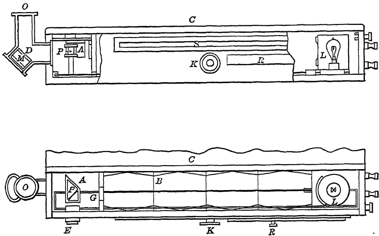
FIG. 50.—Plan and elevation of Sharp-Millar photometer.
