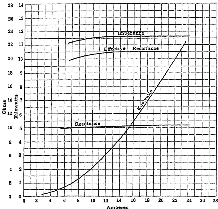
FIG. 4.—Constants for one mile of No. 6 B.W.G. solid BB galvanized iron wire at 60 cycles per second. Direct-current resistance per mile of wire is 10.6 ohms. Tests made on three-phase circuits with wire at vertices of 84-inch equilateral triangle.
