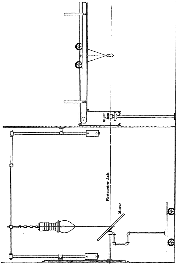
FIG. 53.—One-mirror crane photometer for arc lights.
