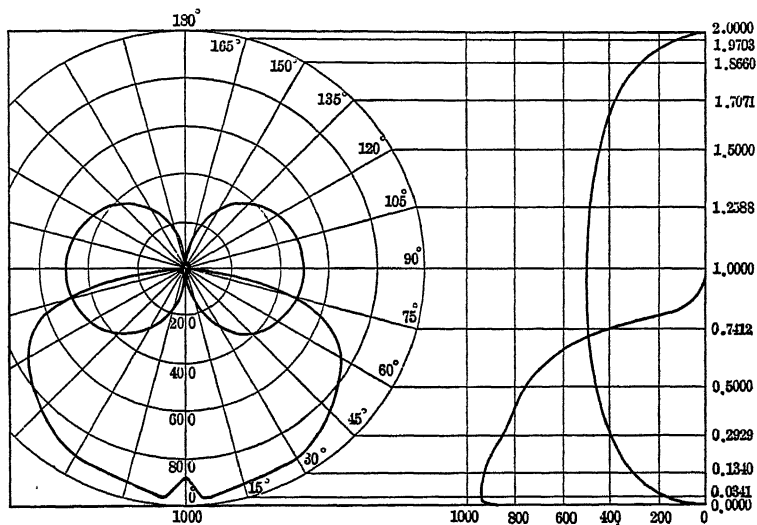
FIG. 58.—Double Rousseau diagram.
