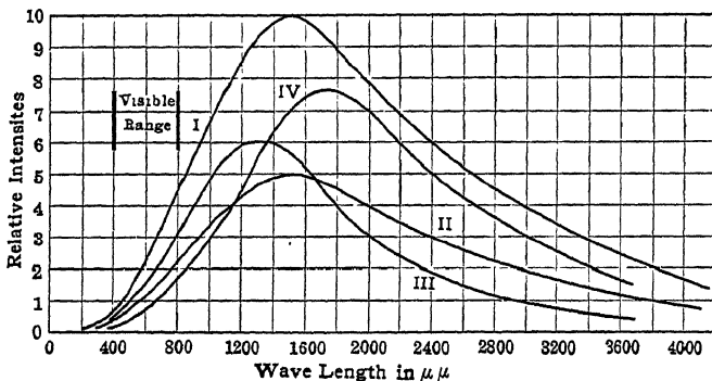
FIG. 35.—Types of energy radiation.
