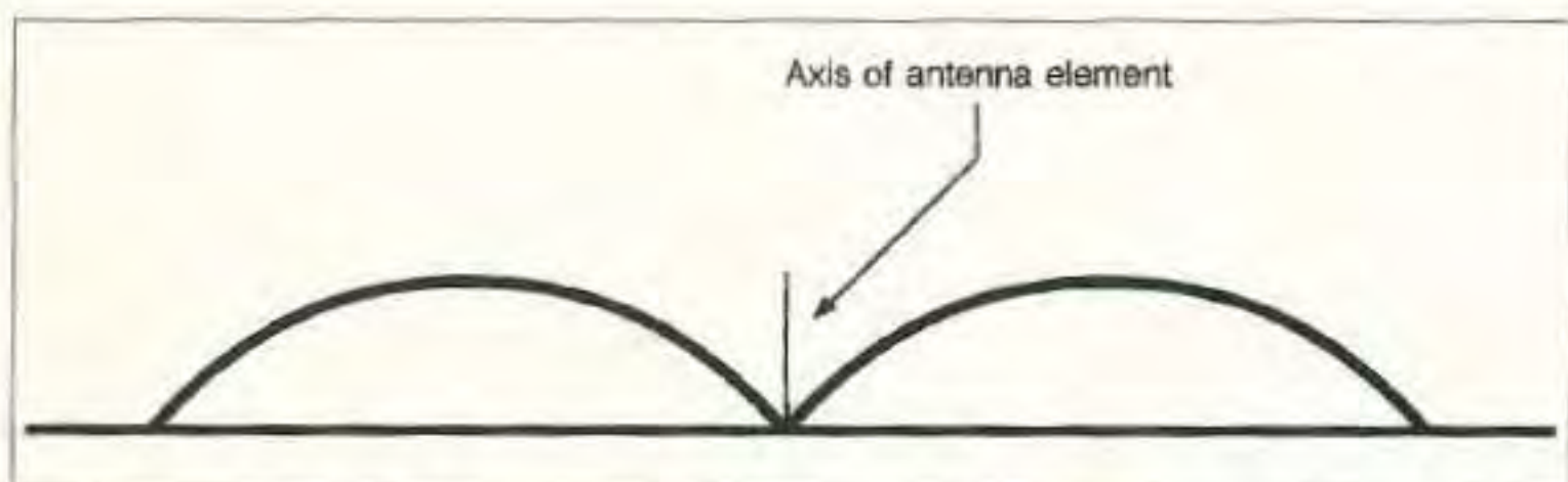
Fig. 6. Idealized vertically compressed radiation pattern of a 1/4-wave gain-designed antenna.
