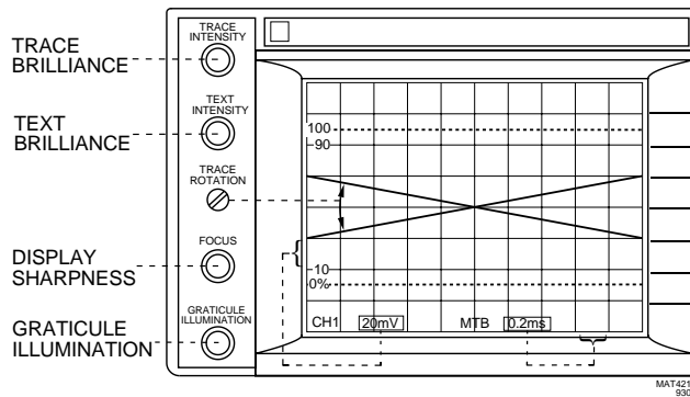
Screen controls and function of TRACE ROTATION.
