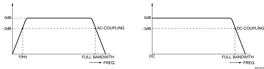
Effect of ac/dc input coupling
