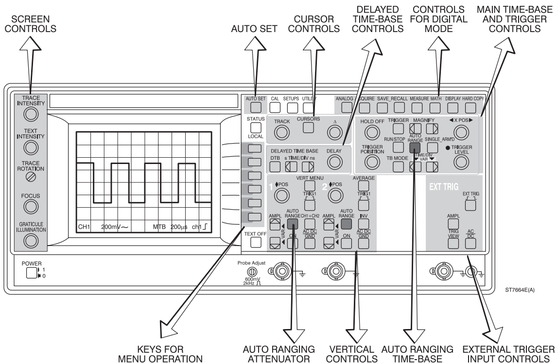
Figure 3.1 Front panel layout
