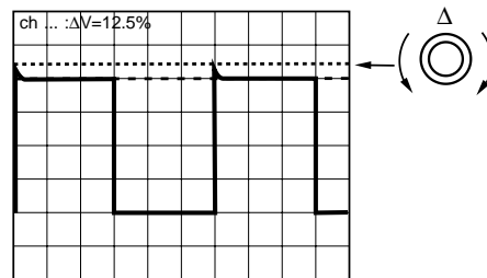
-POSITION \Delta CURSOR ON TOP OF OVERSHOOT
