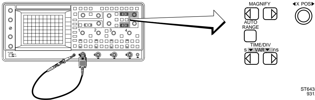
Figure 3.6 Timebase setup
