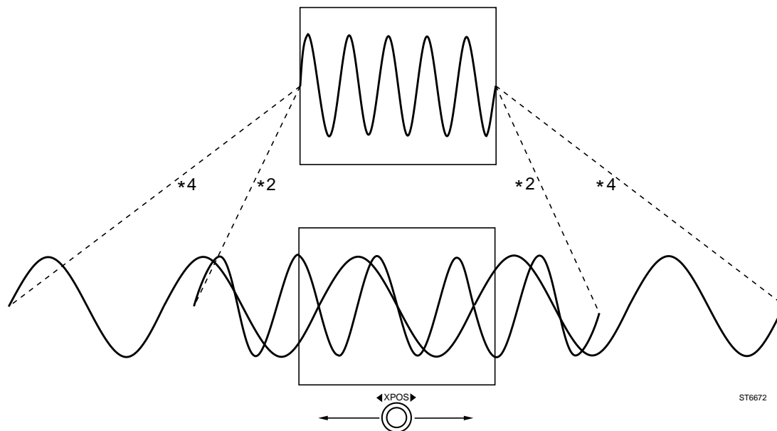
Function of the timebase magnifier and X POS control
