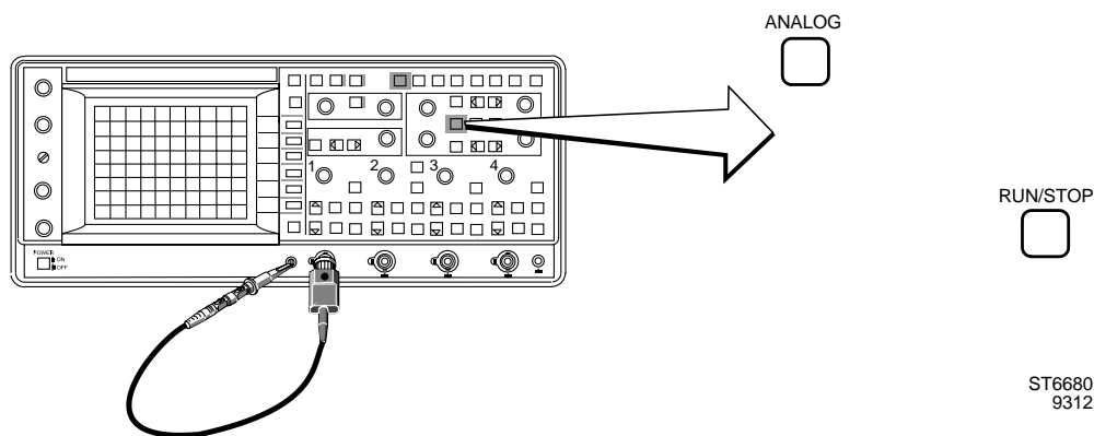
Figure 3.4 Analog-Digital switching setup
