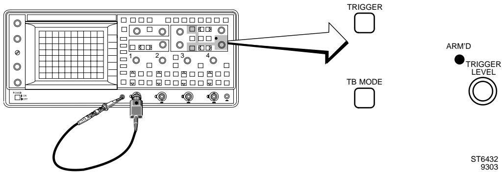
Figure 3.10 More advanced trigger setup
