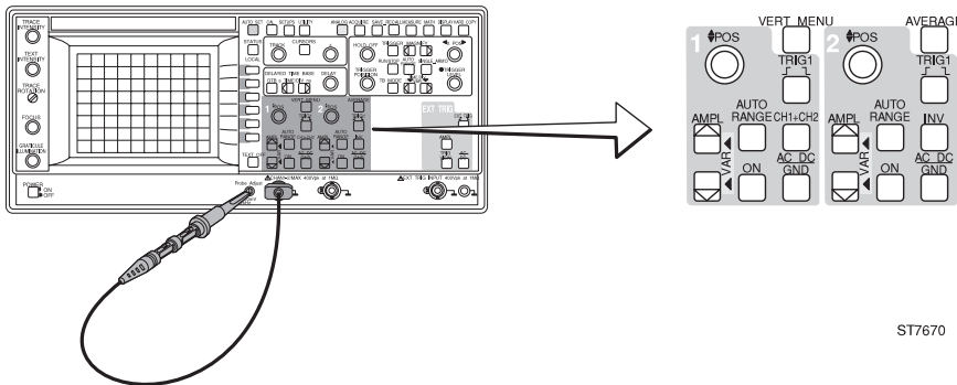
Figure 3.5 Vertical setup
