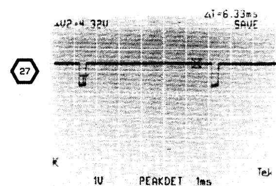
TEST SCOPE TRIGGERED ON U506 PIN 3 FOR WAVEFORMS 27 THROUGH 30
