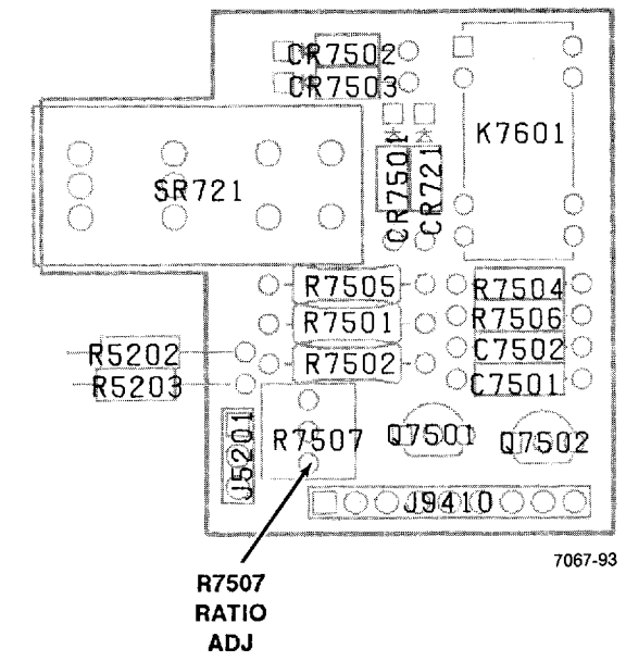
Figure 9-30. A16—Sweep Reference board adjustment locations.
