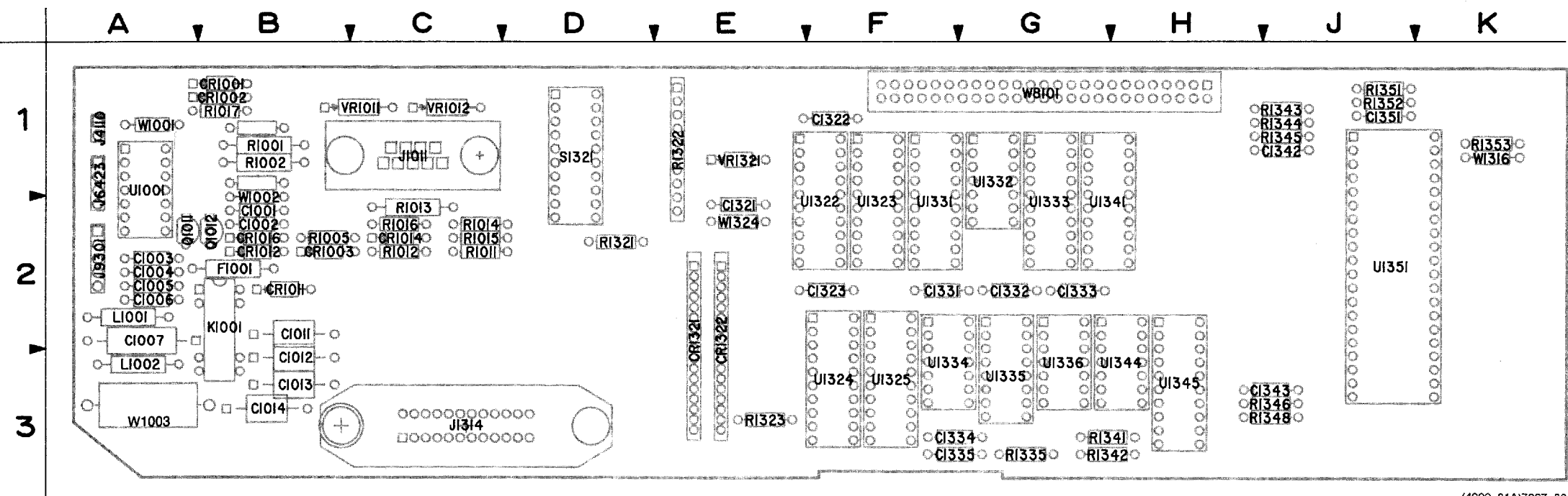
Figure 9-25. A22—GPIB Option board.
