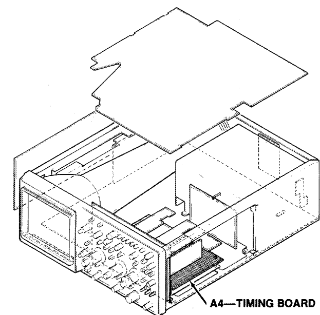
Figure 9-15. A4—Timing board.
