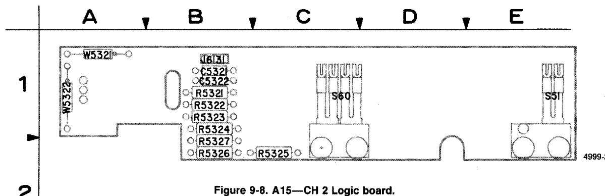
Figure 9-8. A15—CH 2 Logic board.
