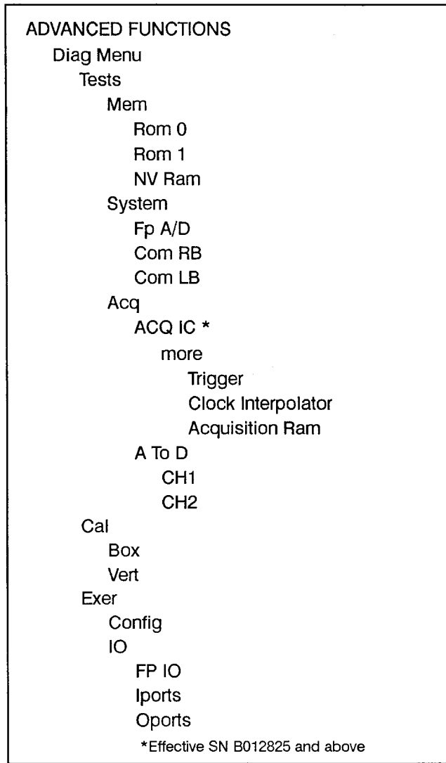
Figure 6-4. Diagnostic Menu Map.
