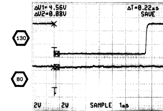
TEST SCOPE TRIGGERED ON U4229 PIN 7, SET TRIGGER SLOPE TO NEGATIVE POLARITY FOR WAVEFORMS 80 THROUGH 93
