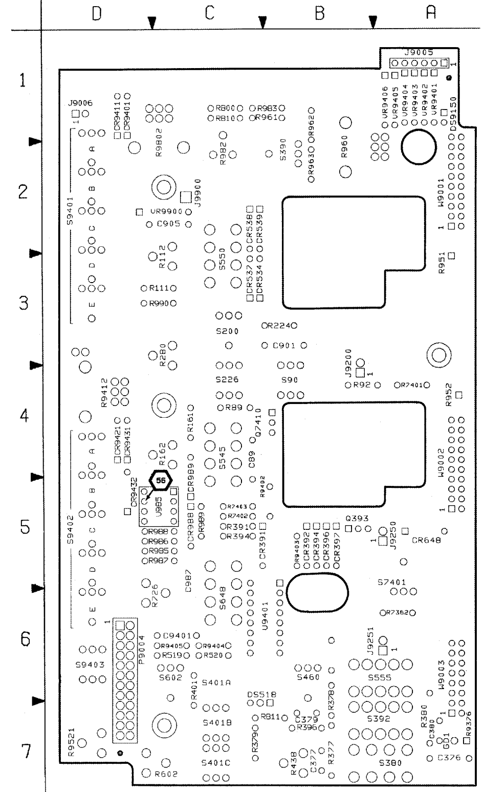
Figure 9-14. Circuit view of A3—Front Panel board.
