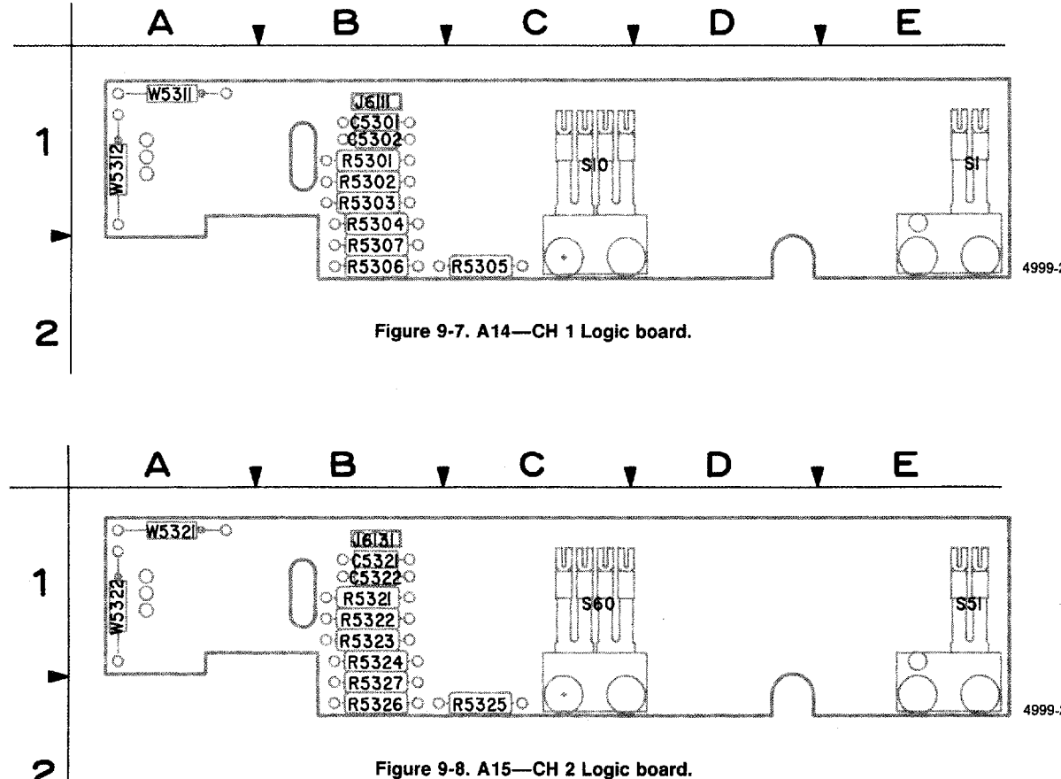
Figure 9-8. A15—CH 2 Logic board.
