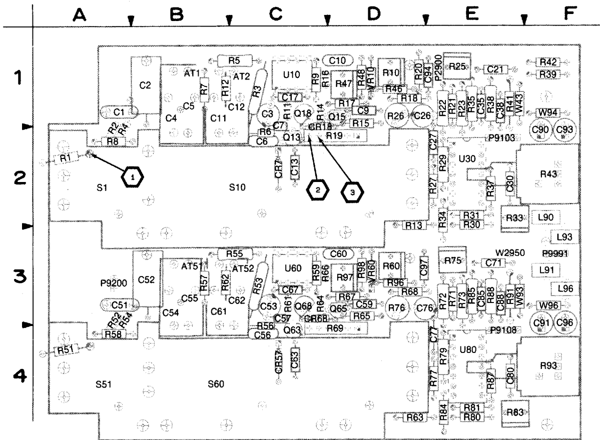
Figure 9-6. A2—Attenuator board.
