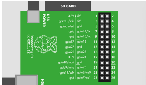
Figure C-3. The GPIO pin header
