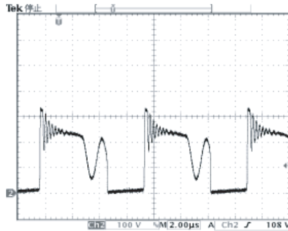
< Vds Voltage Waveform on Sub-power Circuit FET >
